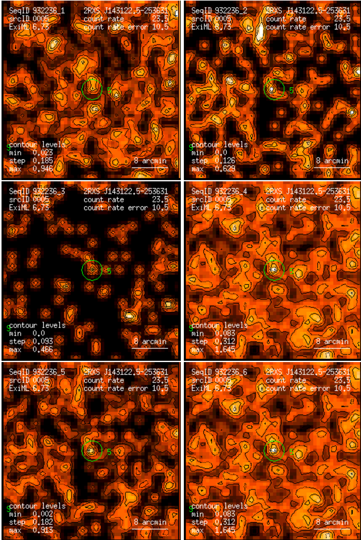
Figure 5: RASS 932236: detection 0005: band rate images, Gaussian filter: (1) PSPC channels 11 – 41, (2) 52 – 90, (3) 91 – 201, (4) 11 – 235, (5) 52 – 201, (6) 11 – 201. Broad band rates in counts/ks. Band rate contour levels in counts/ks/arcmin 2 .
