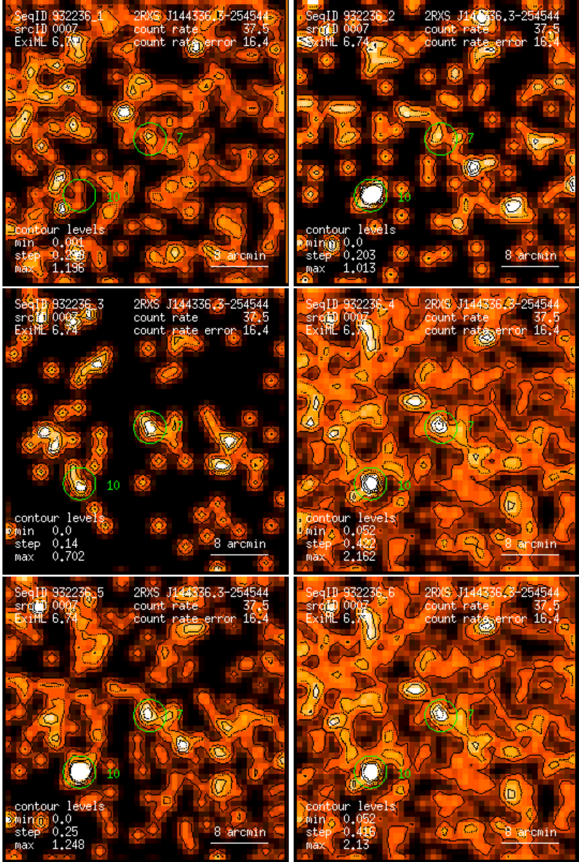
Figure 7: RASS 932236: detection 0007: band rate images, Gaussian filter: (1) PSPC channels 11 – 41, (2) 52 – 90, (3) 91 – 201, (4) 11 – 235, (5) 52 – 201, (6) 11 – 201. Broad band rates in counts/ks. Band rate contour levels in counts/ks/arcmin 2 .
