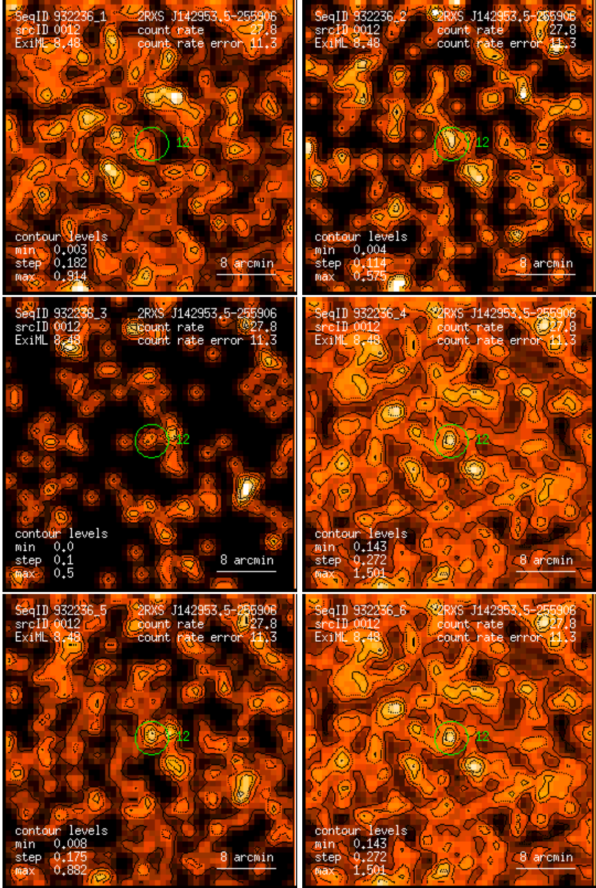
Figure 12: RASS 932236: detection 0012: band rate images, Gaussian filter: (1) PSPC channels 11 – 41, (2) 52 – 90, (3) 91 – 201, (4) 11 – 235, (5) 52 – 201, (6) 11 – 201. Broad band rates in counts/ks. Band rate contour levels in counts/ks/arcmin 2 .
