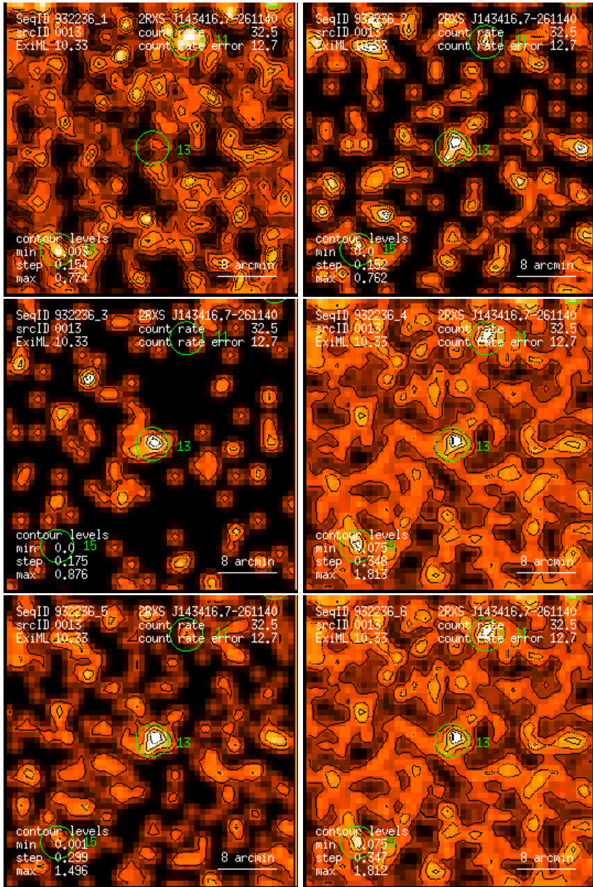
Figure 13: RASS 932236: detection 0013: band rate images, Gaussian filter: (1) PSPC channels 11 – 41, (2) 52 – 90, (3) 91 – 201, (4) 11 – 235, (5) 52 – 201, (6) 11 – 201. Broad band rates in counts/ks. Band rate contour levels in counts/ks/arcmin 2 .
