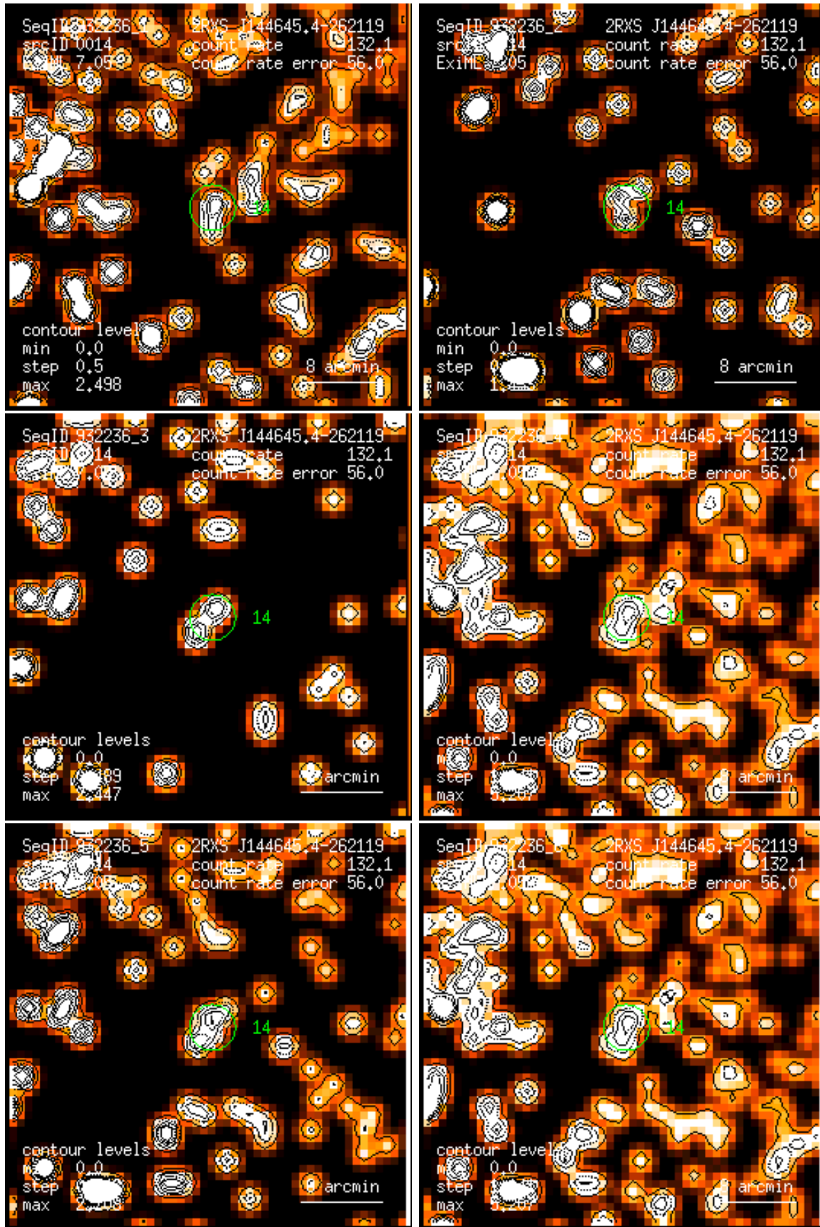
Figure 14: RASS 932236: detection 0014: band rate images, Gaussian filter: (1) PSPC channels 11 – 41, (2) 52 – 90, (3) 91 – 201, (4) 11 – 235, (5) 52 – 201, (6) 11 – 201. Broad band rates in counts/ks. Band rate contour levels in counts/ks/arcmin 2 .
