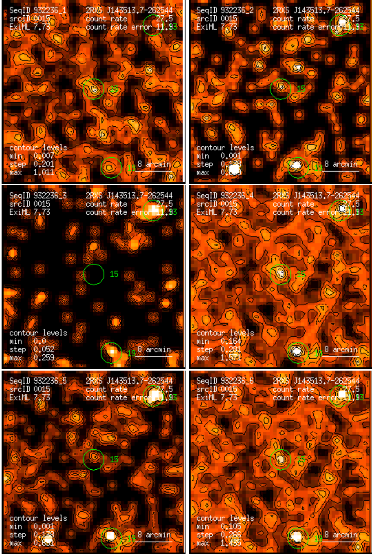
Figure 15: RASS 932236: detection 0015: band rate images, Gaussian filter: (1) PSPC channels 11 – 41, (2) 52 – 90, (3) 91 – 201, (4) 11 – 235, (5) 52 – 201, (6) 11 – 201. Broad band rates in counts/ks. Band rate contour levels in counts/ks/arcmin 2 .
