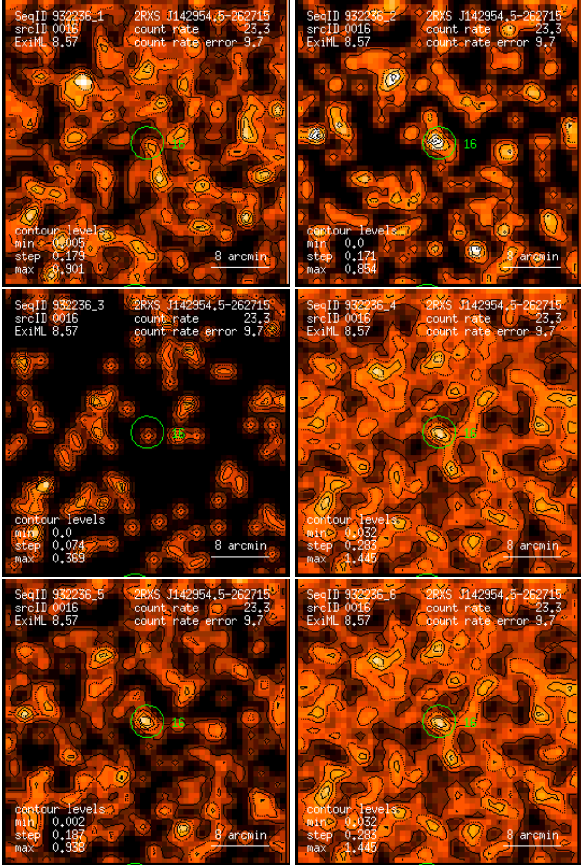
Figure 16: RASS 932236: detection 0016: band rate images, Gaussian filter: (1) PSPC channels 11 – 41, (2) 52 – 90, (3) 91 – 201, (4) 11 – 235, (5) 52 – 201, (6) 11 – 201. Broad band rates in counts/ks. Band rate contour levels in counts/ks/arcmin 2 .
