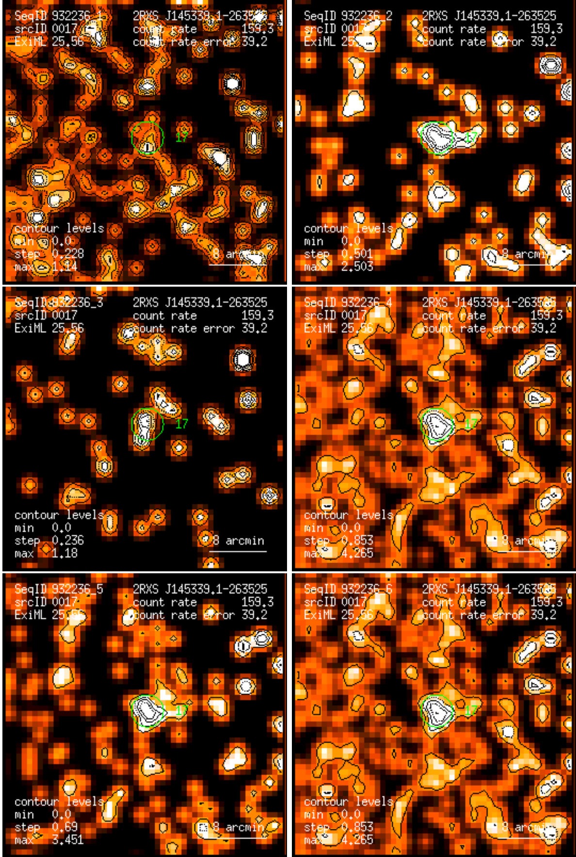
Figure 17: RASS 932236: detection 0017: band rate images, Gaussian filter: (1) PSPC channels 11 – 41, (2) 52 – 90, (3) 91 – 201, (4) 11 – 235, (5) 52 – 201, (6) 11 – 201. Broad band rates in counts/ks. Band rate contour levels in counts/ks/arcmin 2 .
