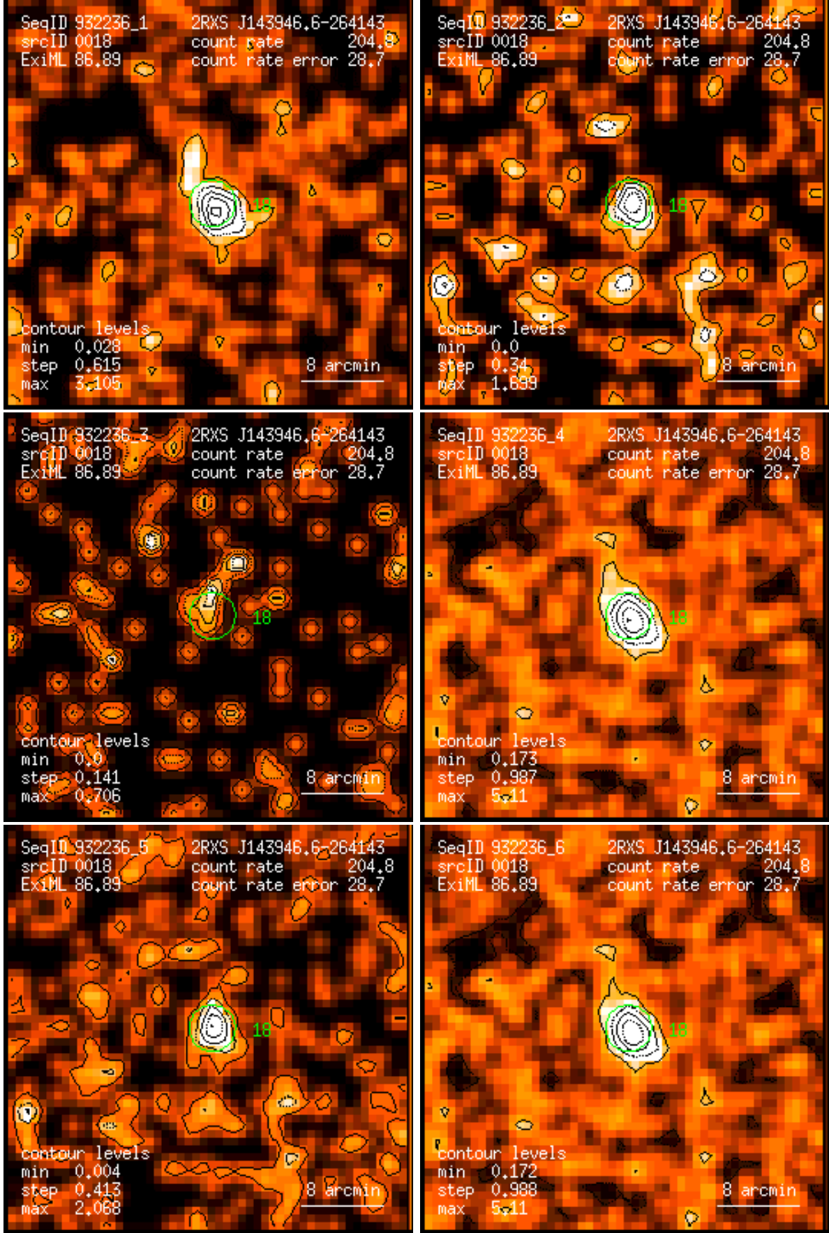
Figure 18: RASS 932236: detection 0018: band rate images, Gaussian filter: (1) PSPC channels 11 – 41, (2) 52 – 90, (3) 91 – 201, (4) 11 – 235, (5) 52 – 201, (6) 11 – 201. Broad band rates in counts/ks. Band rate contour levels in counts/ks/arcmin 2 .
