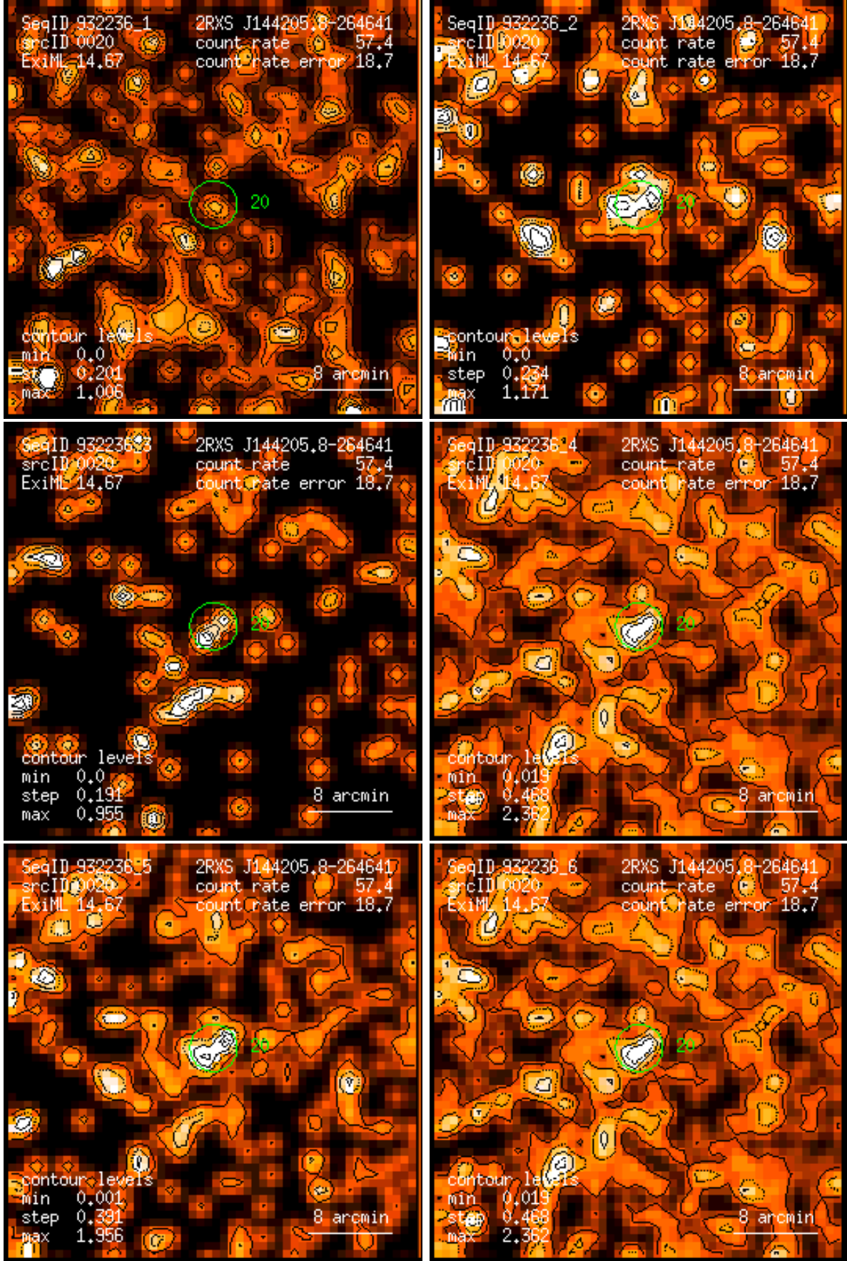
Figure 20: RASS 932236: detection 0020: band rate images, Gaussian filter: (1) PSPC channels 11 – 41, (2) 52 – 90, (3) 91 – 201, (4) 11 – 235, (5) 52 – 201, (6) 11 – 201. Broad band rates in counts/ks. Band rate contour levels in counts/ks/arcmin 2 .
