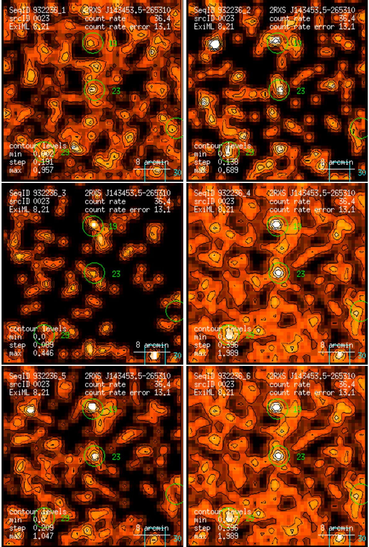
Figure 23: RASS 932236: detection 0023: band rate images, Gaussian filter: (1) PSPC channels 11 – 41, (2) 52 – 90, (3) 91 – 201, (4) 11 – 235, (5) 52 – 201, (6) 11 – 201. Broad band rates in counts/ks. Band rate contour levels in counts/ks/arcmin 2 .
