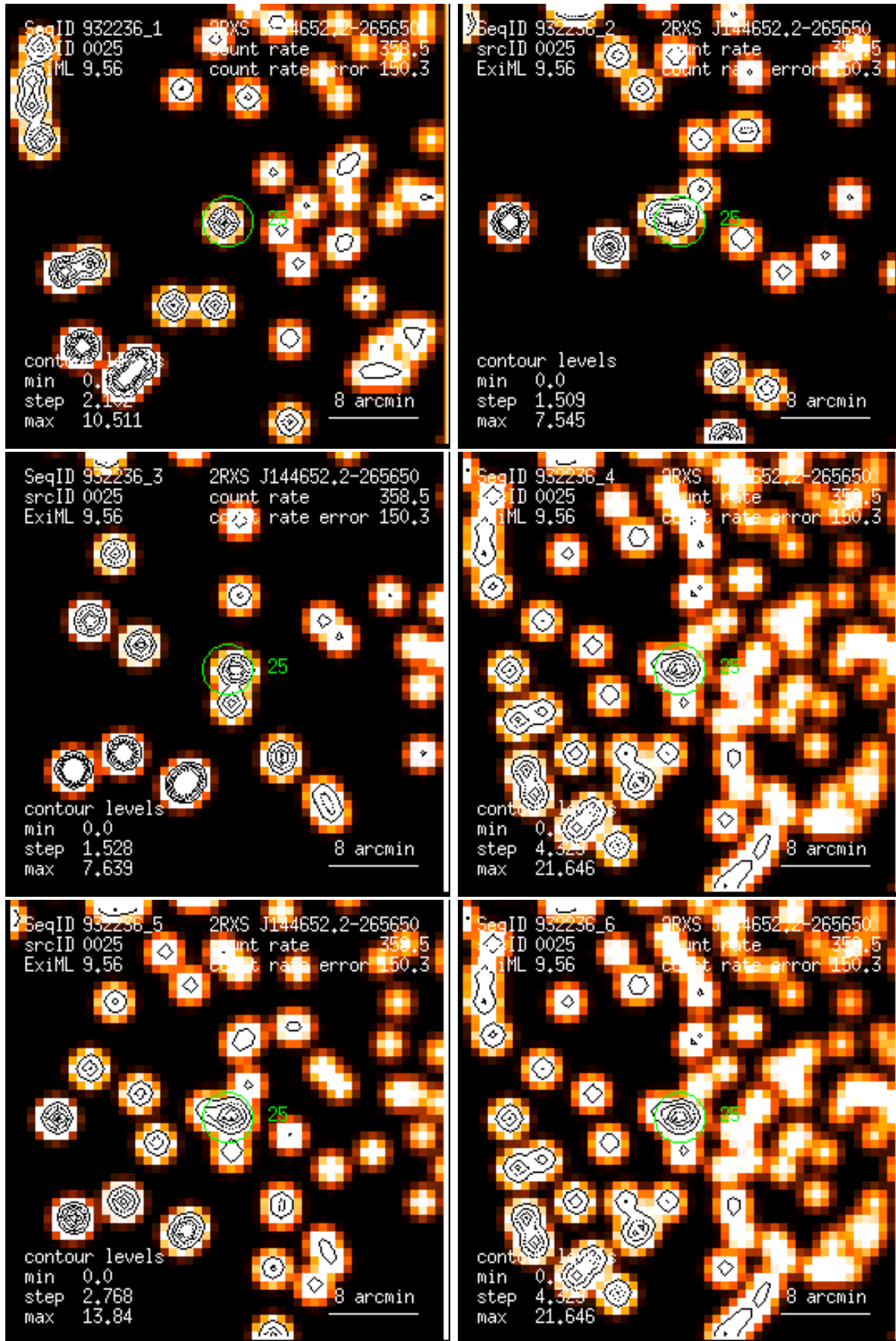
Figure 25: RASS 932236: detection 0025: band rate images, Gaussian filter: (1) PSPC channels 11 – 41, (2) 52 – 90, (3) 91 – 201, (4) 11 – 235, (5) 52 – 201, (6) 11 – 201. Broad band rates in counts/ks. Band rate contour levels in counts/ks/arcmin 2 .
