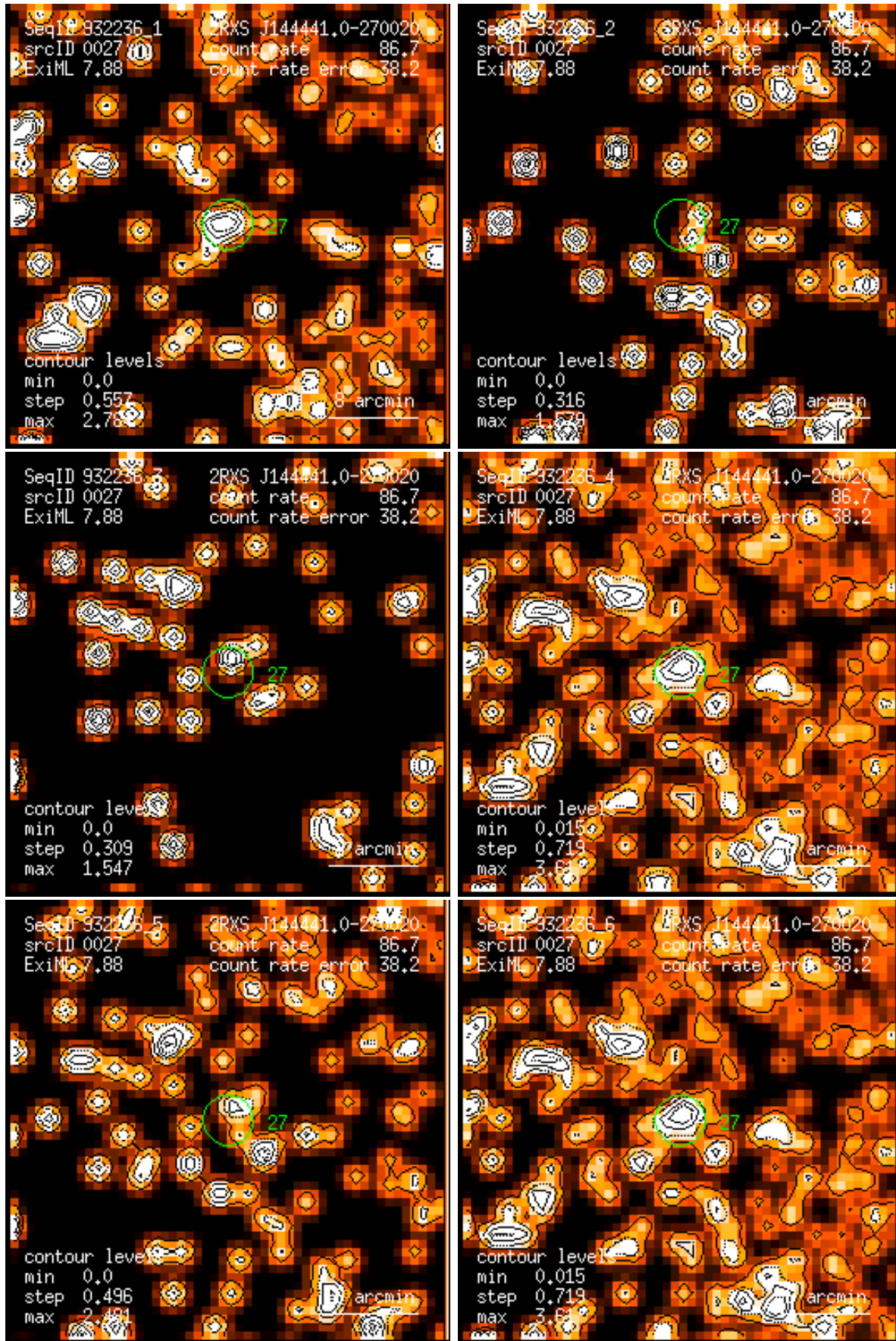
Figure 27: RASS 932236: detection 0027: band rate images, Gaussian filter: (1) PSPC channels 11 – 41, (2) 52 – 90, (3) 91 – 201, (4) 11 – 235, (5) 52 – 201, (6) 11 – 201. Broad band rates in counts/ks. Band rate contour levels in counts/ks/arcmin 2 .
