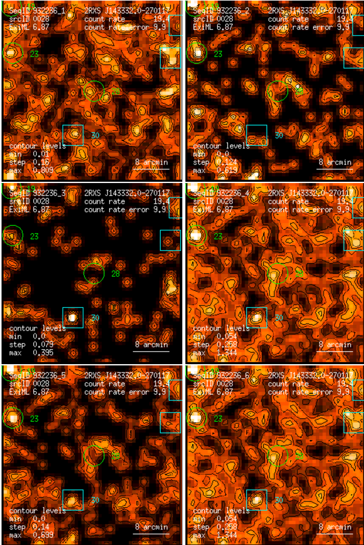
Figure 28: RASS 932236: detection 0028: band rate images, Gaussian filter: (1) PSPC channels 11 – 41, (2) 52 – 90, (3) 91 – 201, (4) 11 – 235, (5) 52 – 201, (6) 11 – 201. Broad band rates in counts/ks. Band rate contour levels in counts/ks/arcmin 2 .
