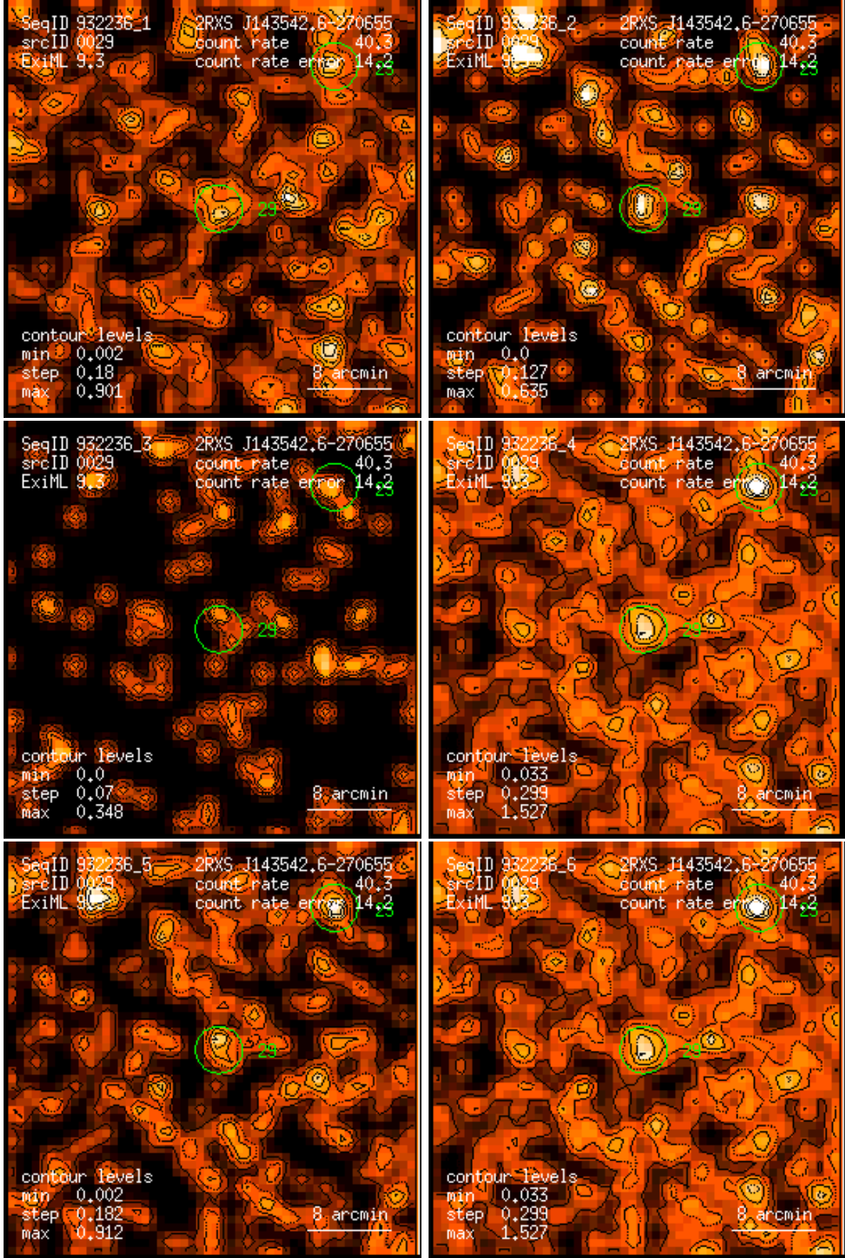
Figure 29: RASS 932236: detection 0029: band rate images, Gaussian filter: (1) PSPC channels 11 – 41, (2) 52 – 90, (3) 91 – 201, (4) 11 – 235, (5) 52 – 201, (6) 11 – 201. Broad band rates in counts/ks. Band rate contour levels in counts/ks/arcmin 2 .
