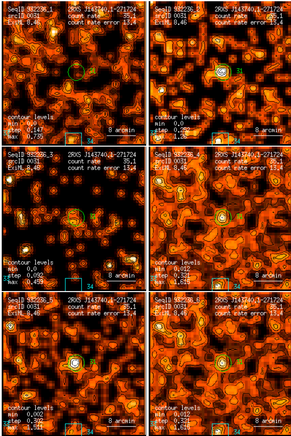
Figure 31: RASS 932236: detection 0031: band rate images, Gaussian filter: (1) PSPC channels 11 – 41, (2) 52 – 90, (3) 91 – 201, (4) 11 – 235, (5) 52 – 201, (6) 11 – 201. Broad band rates in counts/ks. Band rate contour levels in counts/ks/arcmin 2 .
