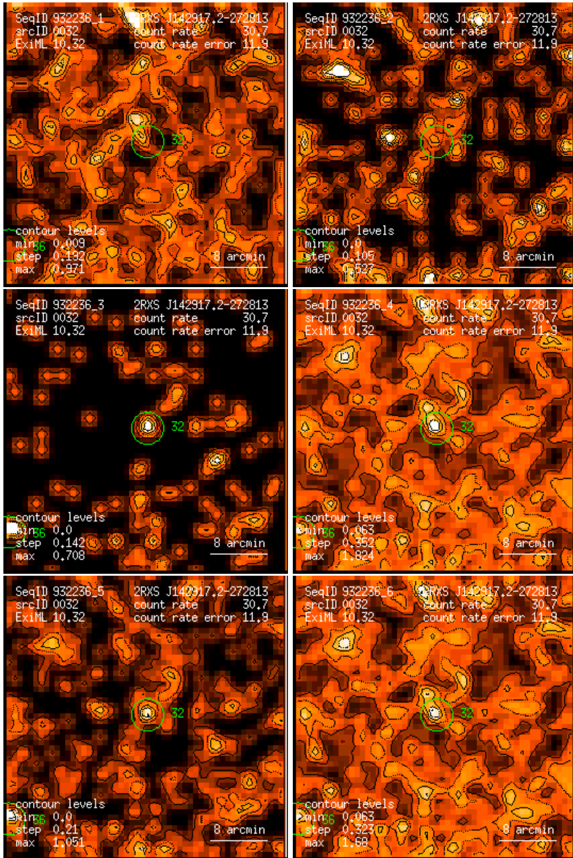
Figure 32: RASS 932236: detection 0032: band rate images, Gaussian filter: (1) PSPC channels 11 – 41, (2) 52 – 90, (3) 91 – 201, (4) 11 – 235, (5) 52 – 201, (6) 11 – 201. Broad band rates in counts/ks. Band rate contour levels in counts/ks/arcmin 2 .
