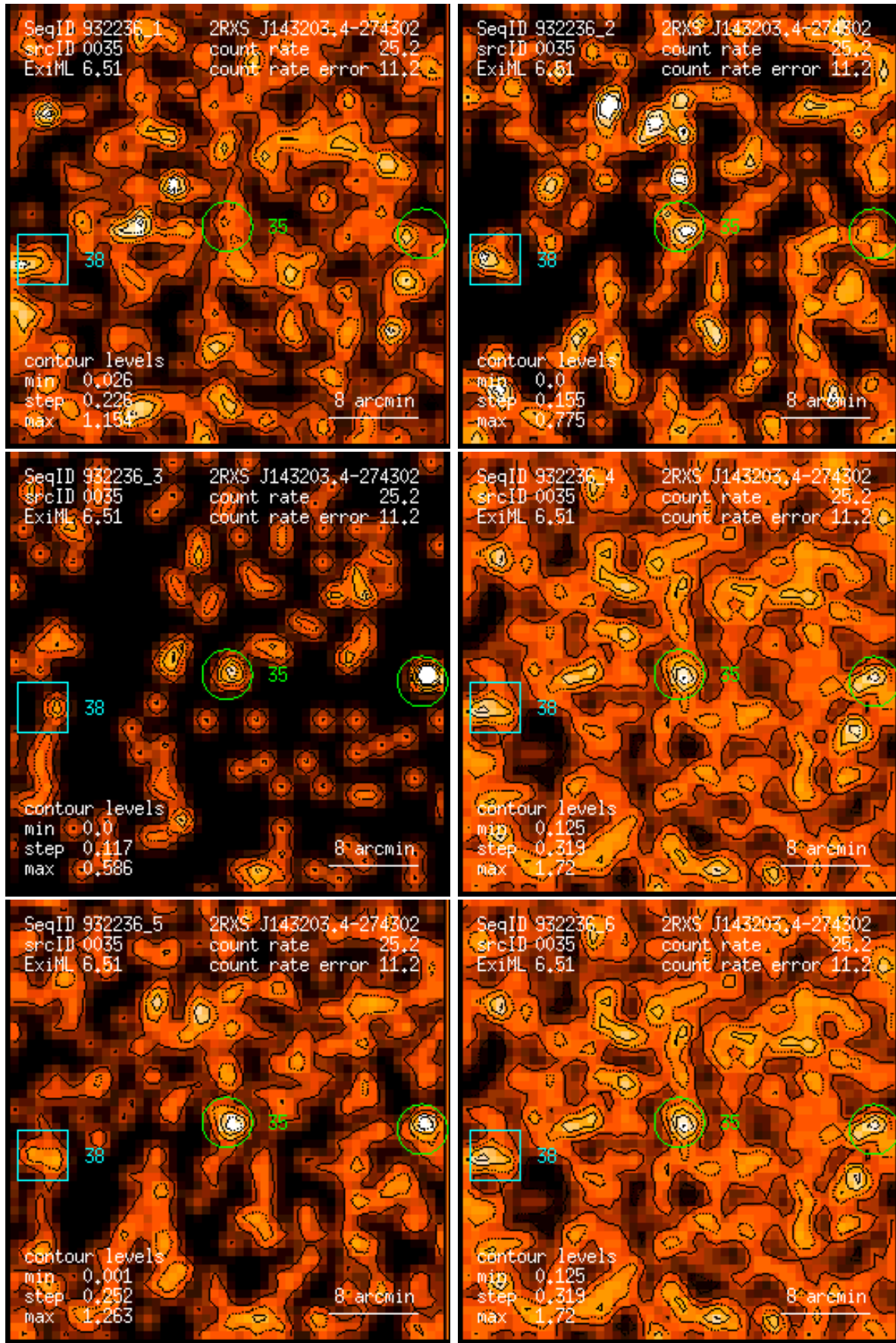
Figure 35: RASS 932236: detection 0035: band rate images, Gaussian filter: (1) PSPC channels 11 – 41, (2) 52 – 90, (3) 91 – 201, (4) 11 – 235, (5) 52 – 201, (6) 11 – 201. Broad band rates in counts/ks. Band rate contour levels in counts/ks/arcmin 2 .
