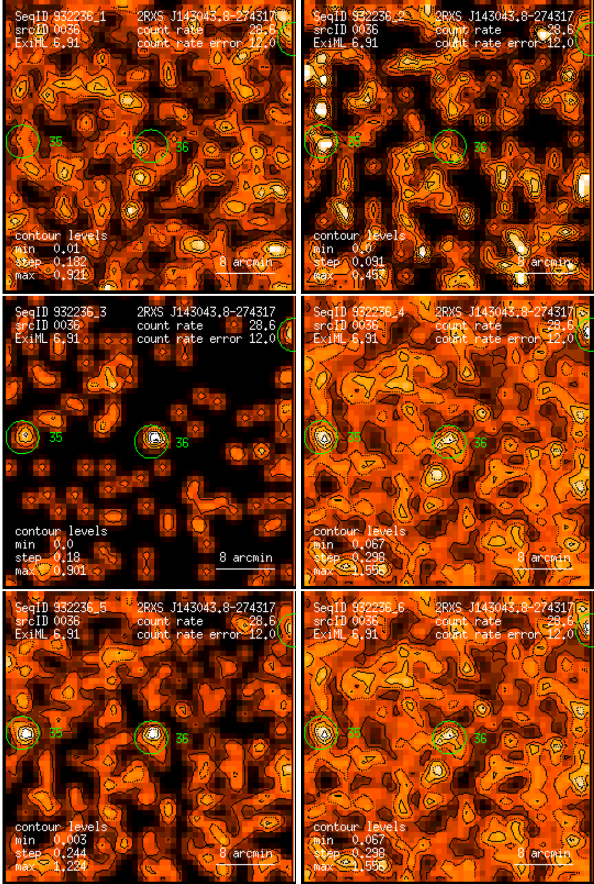
Figure 36: RASS 932236: detection 0036: band rate images, Gaussian filter: (1) PSPC channels 11 – 41, (2) 52 – 90, (3) 91 – 201, (4) 11 – 235, (5) 52 – 201, (6) 11 – 201. Broad band rates in counts/ks. Band rate contour levels in counts/ks/arcmin 2 .
