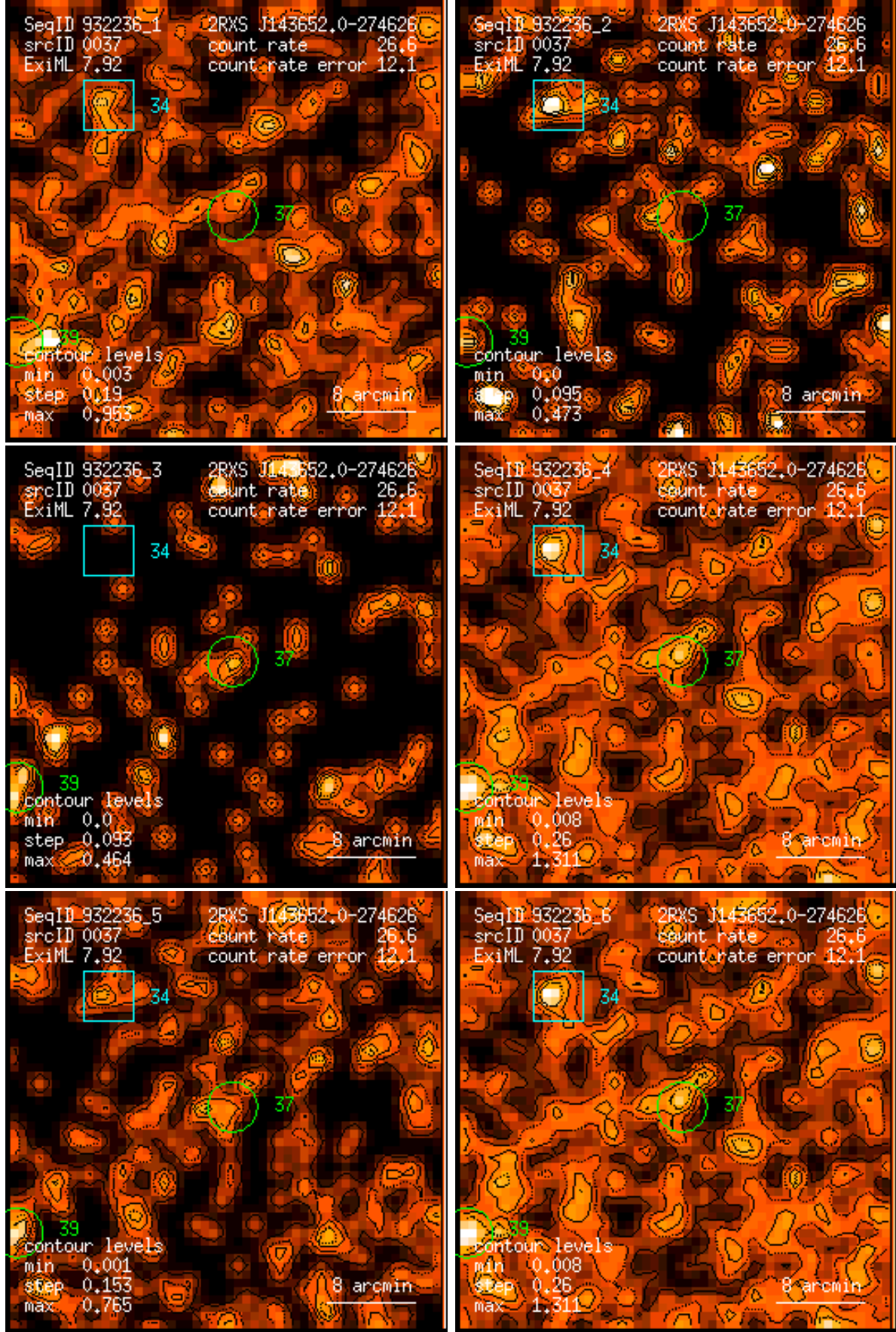
Figure 37: RASS 932236: detection 0037: band rate images, Gaussian filter: (1) PSPC channels 11 – 41, (2) 52 – 90, (3) 91 – 201, (4) 11 – 235, (5) 52 – 201, (6) 11 – 201. Broad band rates in counts/ks. Band rate contour levels in counts/ks/arcmin 2 .
