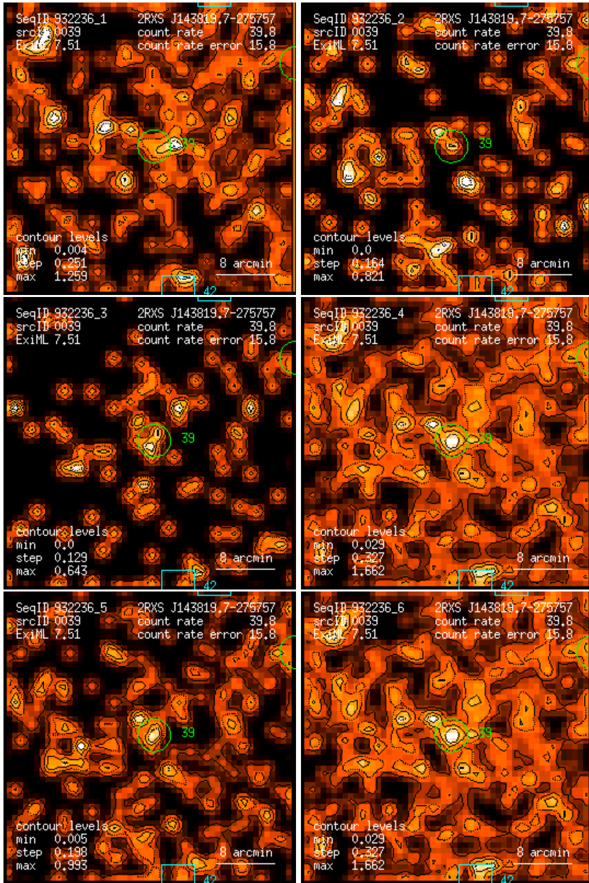
Figure 39: RASS 932236: detection 0039: band rate images, Gaussian filter: (1) PSPC channels 11 – 41, (2) 52 – 90, (3) 91 – 201, (4) 11 – 235, (5) 52 – 201, (6) 11 – 201. Broad band rates in counts/ks. Band rate contour levels in counts/ks/arcmin 2 .
