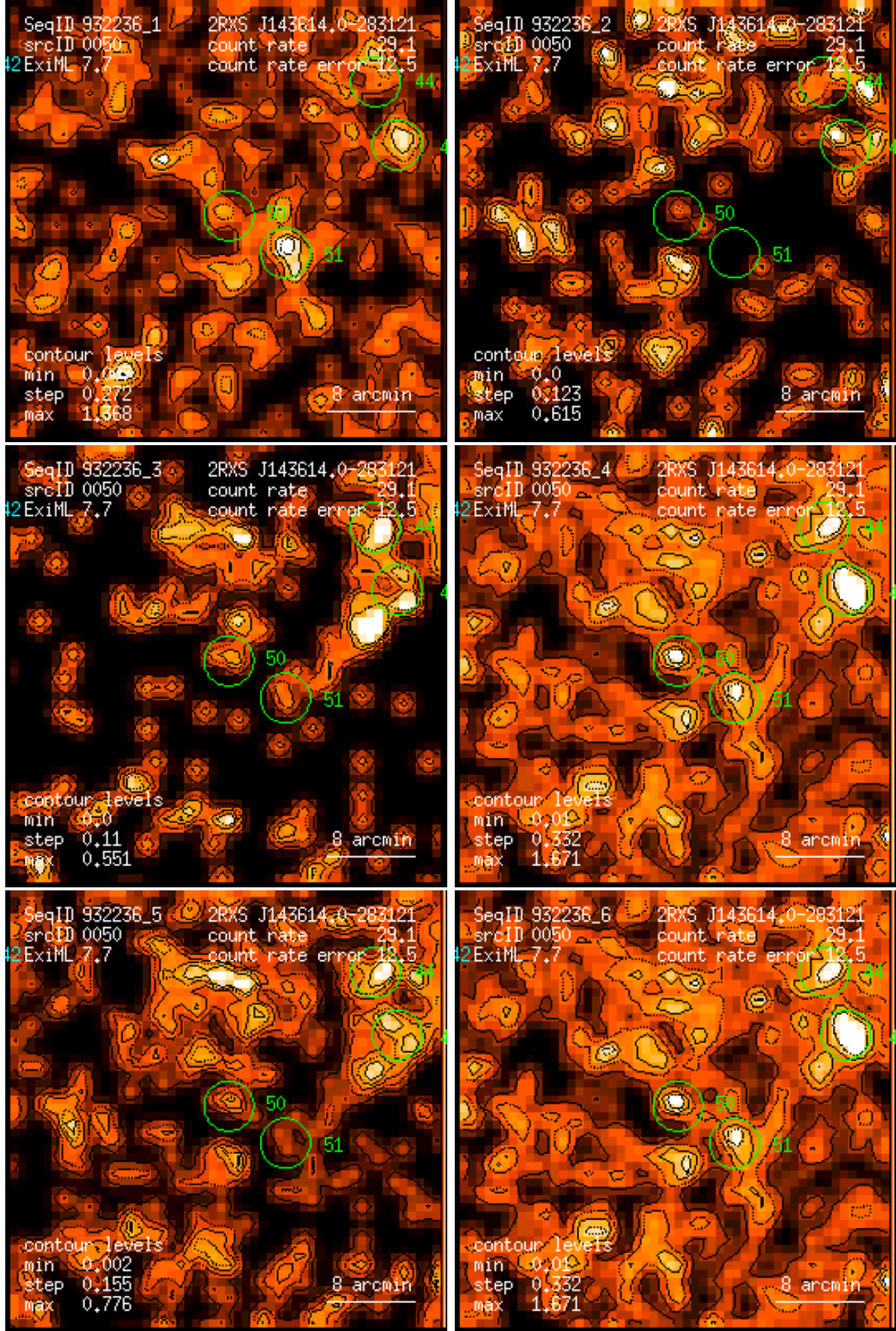
Figure 50: RASS 932236: detection 0050: band rate images, Gaussian filter: (1) PSPC channels 11 – 41, (2) 52 – 90, (3) 91 – 201, (4) 11 – 235, (5) 52 – 201, (6) 11 – 201. Broad band rates in counts/ks. Band rate contour levels in counts/ks/arcmin 2 .
