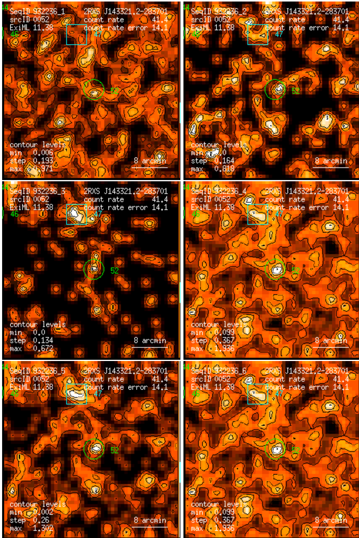
Figure 52: RASS 932236: detection 0052: band rate images, Gaussian filter: (1) PSPC channels 11 – 41, (2) 52 – 90, (3) 91 – 201, (4) 11 – 235, (5) 52 – 201, (6) 11 – 201. Broad band rates in counts/ks. Band rate contour levels in counts/ks/arcmin 2 .
