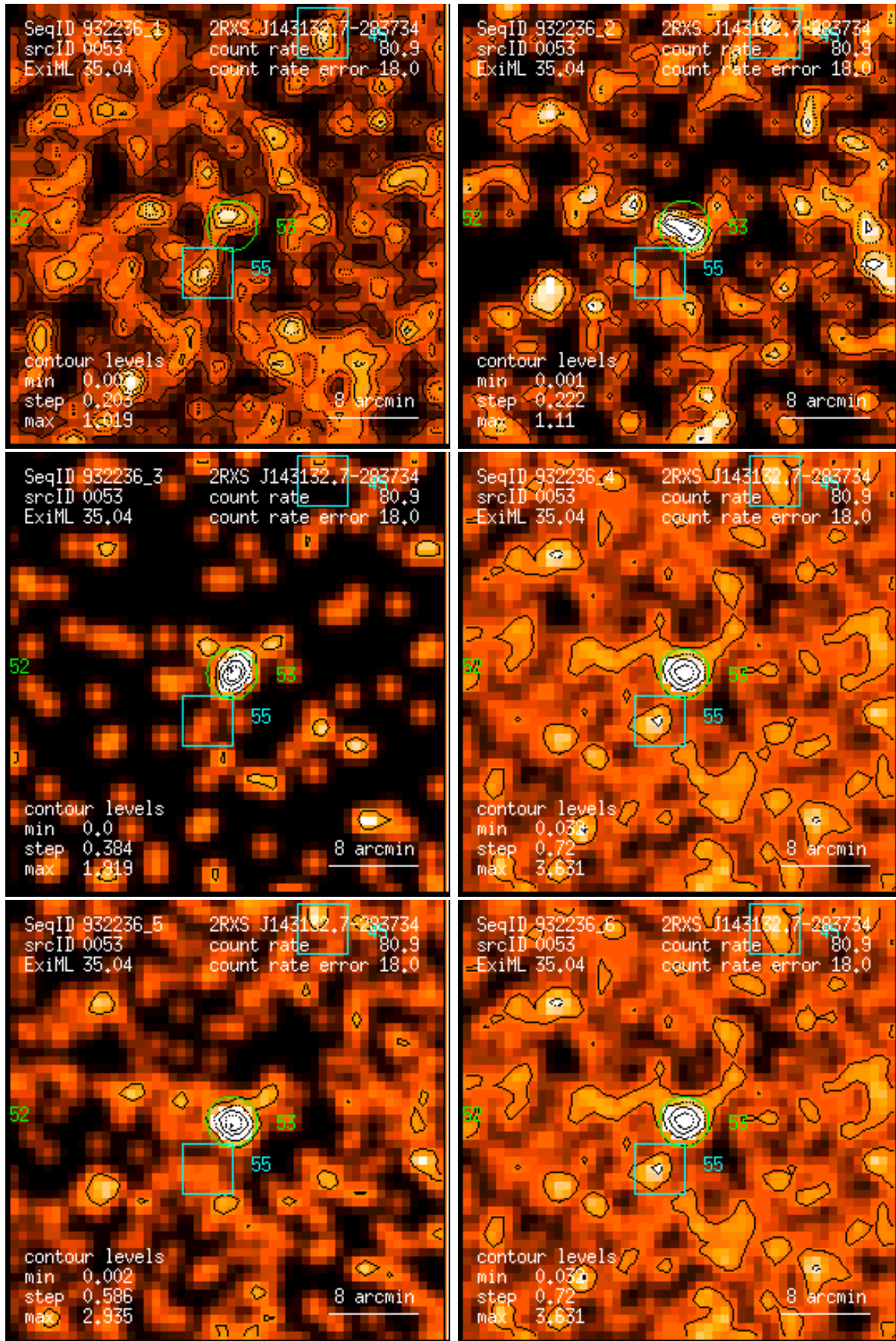
Figure 53: RASS 932236: detection 0053: band rate images, Gaussian filter: (1) PSPC channels 11 – 41, (2) 52 – 90, (3) 91 – 201, (4) 11 – 235, (5) 52 – 201, (6) 11 – 201. Broad band rates in counts/ks. Band rate contour levels in counts/ks/arcmin 2 .
