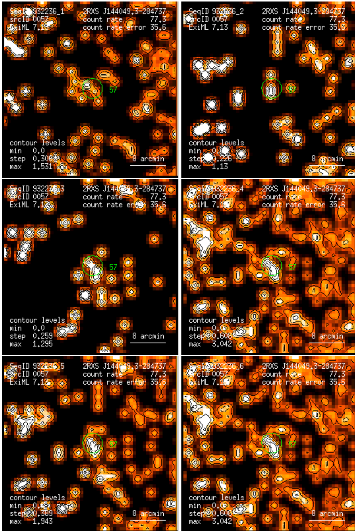
Figure 57: RASS 932236: detection 0057: band rate images, Gaussian filter: (1) PSPC channels 11 – 41, (2) 52 – 90, (3) 91 – 201, (4) 11 – 235, (5) 52 – 201, (6) 11 – 201. Broad band rates in counts/ks. Band rate contour levels in counts/ks/arcmin 2 .
