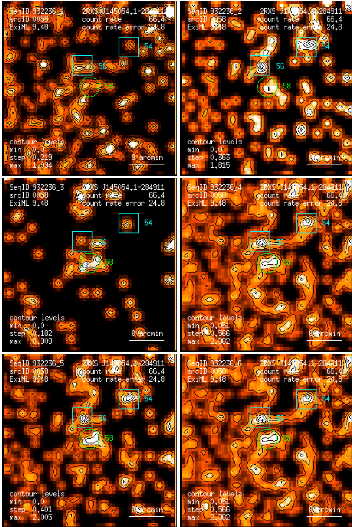
Figure 58: RASS 932236: detection 0058: band rate images, Gaussian filter: (1) PSPC channels 11 – 41, (2) 52 – 90, (3) 91 – 201, (4) 11 – 235, (5) 52 – 201, (6) 11 – 201. Broad band rates in counts/ks. Band rate contour levels in counts/ks/arcmin 2 .
