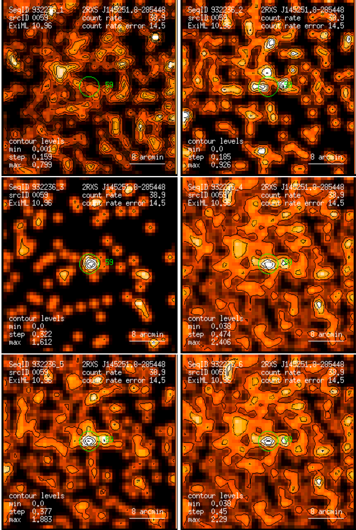
Figure 59: RASS 932236: detection 0059: band rate images, Gaussian filter: (1) PSPC channels 11 – 41, (2) 52 – 90, (3) 91 – 201, (4) 11 – 235, (5) 52 – 201, (6) 11 – 201. Broad band rates in counts/ks. Band rate contour levels in counts/ks/arcmin 2 .
