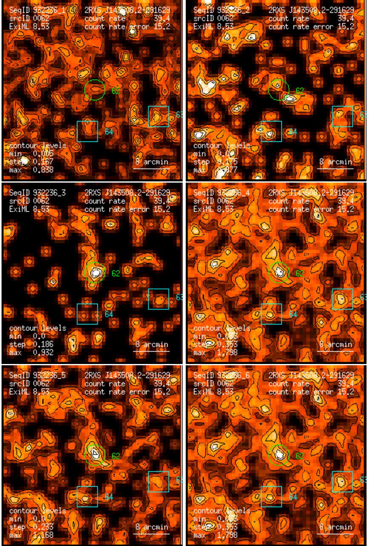
Figure 62: RASS 932236: detection 0062: band rate images, Gaussian filter: (1) PSPC channels 11 – 41, (2) 52 – 90, (3) 91 – 201, (4) 11 – 235, (5) 52 – 201, (6) 11 – 201. Broad band rates in counts/ks. Band rate contour levels in counts/ks/arcmin 2 .
