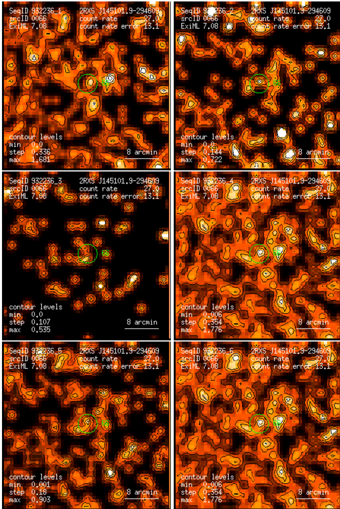
Figure 66: RASS 932236: detection 0066: band rate images, Gaussian filter: (1) PSPC channels 11 – 41, (2) 52 – 90, (3) 91 – 201, (4) 11 – 235, (5) 52 – 201, (6) 11 – 201. Broad band rates in counts/ks. Band rate contour levels in counts/ks/arcmin 2 .
