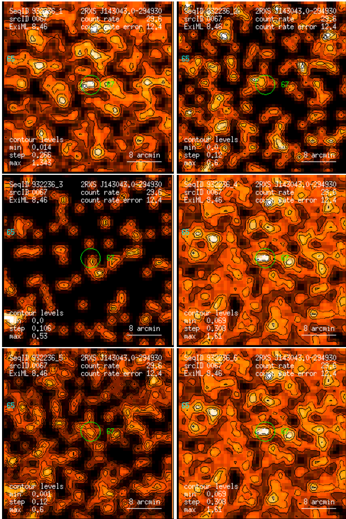
Figure 67: RASS 932236: detection 0067: band rate images, Gaussian filter: (1) PSPC channels 11 – 41, (2) 52 – 90, (3) 91 – 201, (4) 11 – 235, (5) 52 – 201, (6) 11 – 201. Broad band rates in counts/ks. Band rate contour levels in counts/ks/arcmin 2 .
