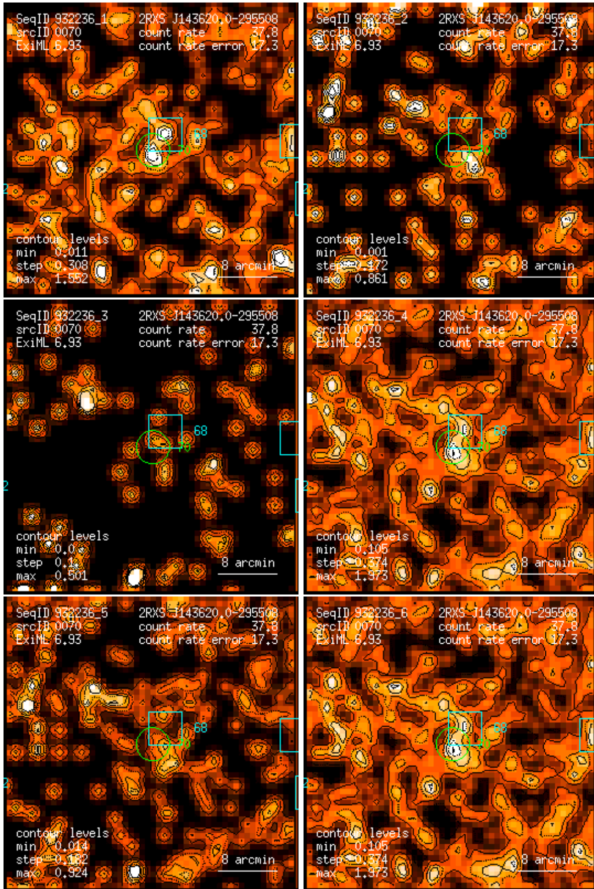
Figure 70: RASS 932236: detection 0070: band rate images, Gaussian filter: (1) PSPC channels 11 – 41, (2) 52 – 90, (3) 91 – 201, (4) 11 – 235, (5) 52 – 201, (6) 11 – 201. Broad band rates in counts/ks. Band rate contour levels in counts/ks/arcmin 2 .
