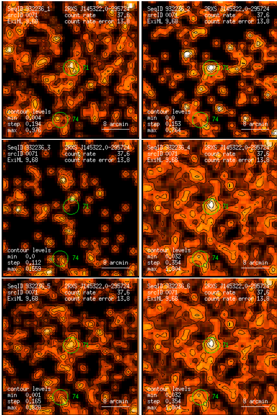
Figure 71: RASS 932236: detection 0071: band rate images, Gaussian filter: (1) PSPC channels 11 – 41, (2) 52 – 90, (3) 91 – 201, (4) 11 – 235, (5) 52 – 201, (6) 11 – 201. Broad band rates in counts/ks. Band rate contour levels in counts/ks/arcmin 2 .
