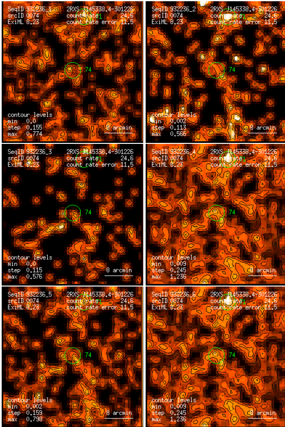
Figure 74: RASS 932236: detection 0074: band rate images, Gaussian filter: (1) PSPC channels 11 – 41, (2) 52 – 90, (3) 91 – 201, (4) 11 – 235, (5) 52 – 201, (6) 11 – 201. Broad band rates in counts/ks. Band rate contour levels in counts/ks/arcmin 2 .
