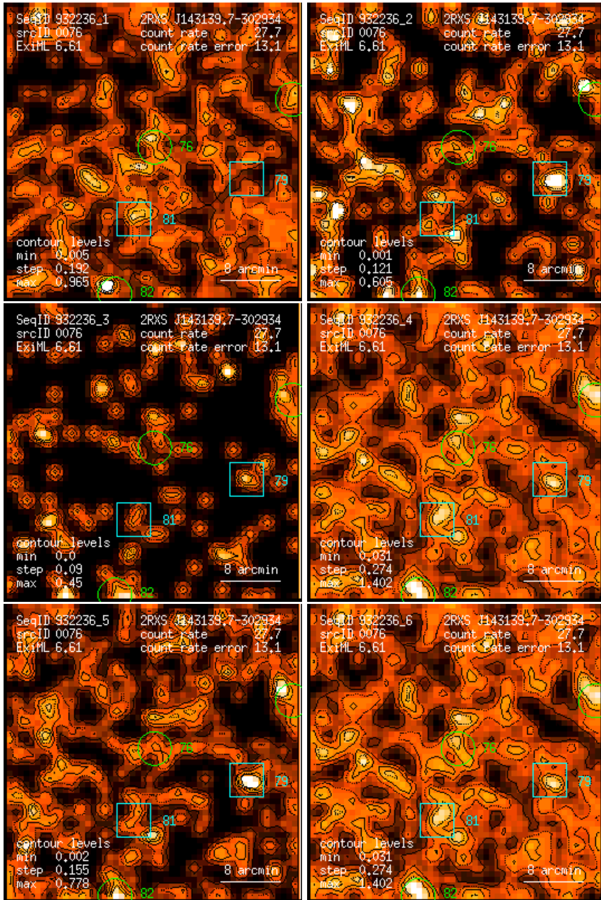
Figure 76: RASS 932236: detection 0076: band rate images, Gaussian filter: (1) PSPC channels 11 – 41, (2) 52 – 90, (3) 91 – 201, (4) 11 – 235, (5) 52 – 201, (6) 11 – 201. Broad band rates in counts/ks. Band rate contour levels in counts/ks/arcmin 2 .
