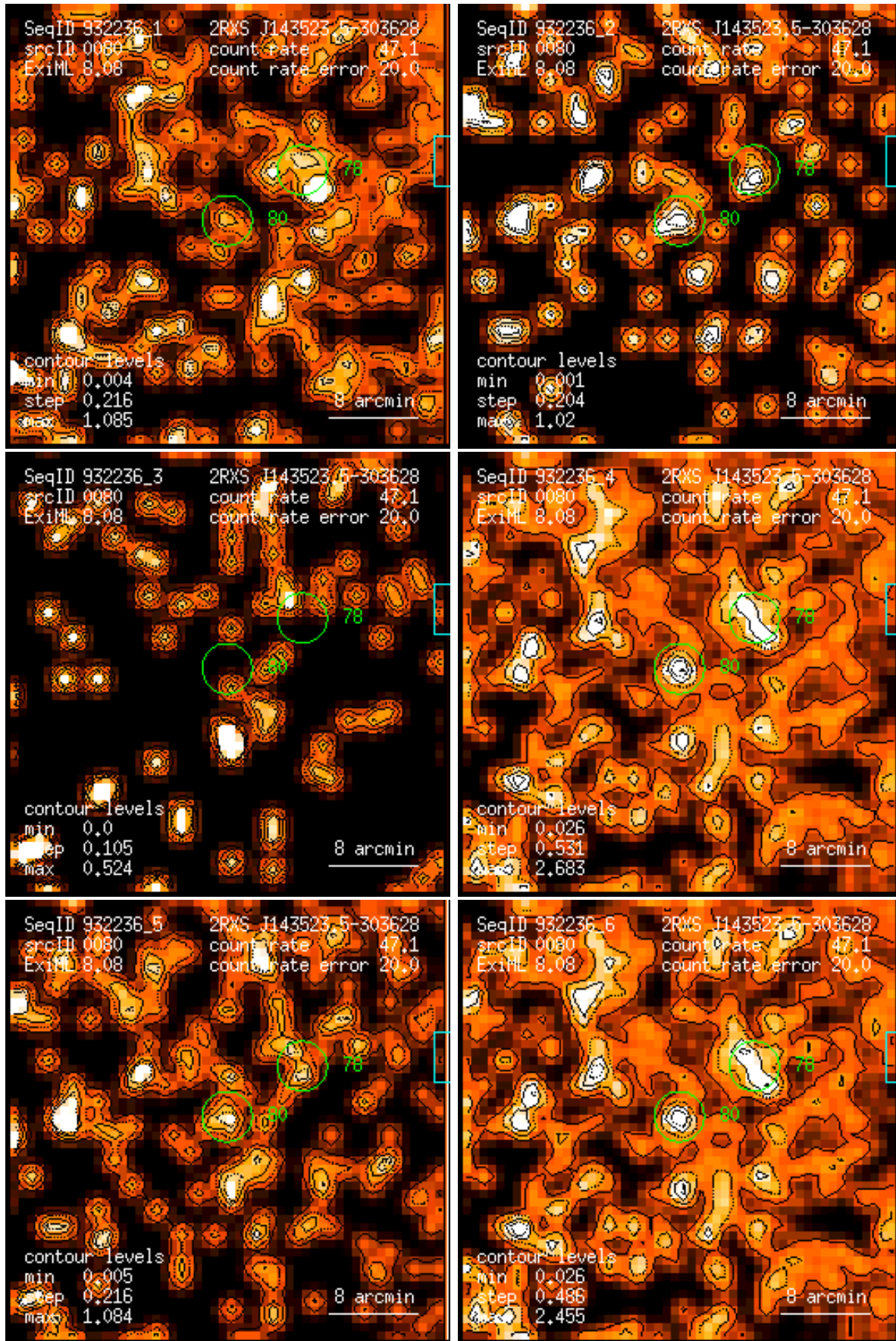
Figure 80: RASS 932236: detection 0080: band rate images, Gaussian filter: (1) PSPC channels 11 – 41, (2) 52 – 90, (3) 91 – 201, (4) 11 – 235, (5) 52 – 201, (6) 11 – 201. Broad band rates in counts/ks. Band rate contour levels in counts/ks/arcmin 2 .
