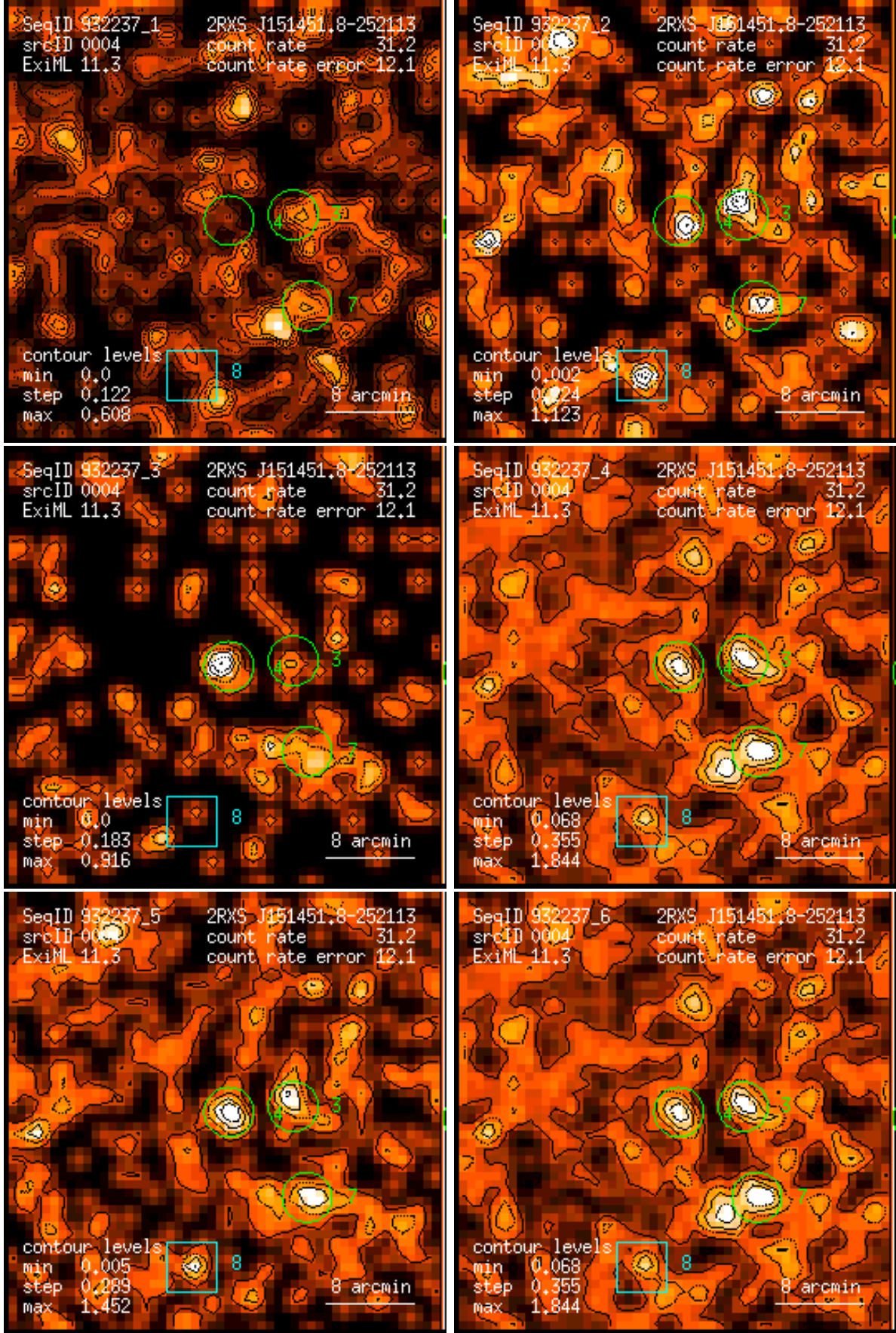
Figure 4: RASS 932237: detection 0004: band rate images, Gaussian filter: (1) PSPC channels 11 – 41, (2) 52 – 90, (3) 91 – 201, (4) 11 – 235, (5) 52 – 201, (6) 11 – 201. Broad band rates in counts/ks. Band rate contour levels in counts/ks/arcmin 2 .
