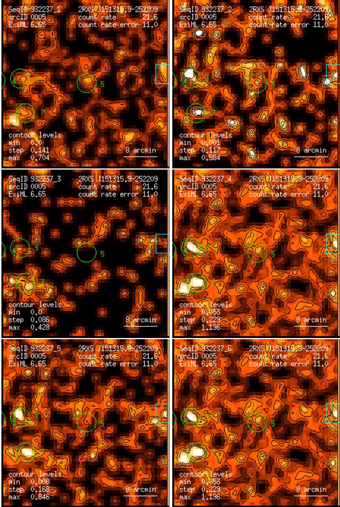
Figure 5: RASS 932237: detection 0005: band rate images, Gaussian filter: (1) PSPC channels 11 – 41, (2) 52 – 90, (3) 91 – 201, (4) 11 – 235, (5) 52 – 201, (6) 11 – 201. Broad band rates in counts/ks. Band rate contour levels in counts/ks/arcmin 2 .
