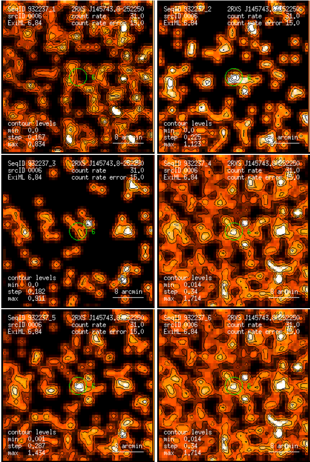
Figure 6: RASS 932237: detection 0006: band rate images, Gaussian filter: (1) PSPC channels 11 – 41, (2) 52 – 90, (3) 91 – 201, (4) 11 – 235, (5) 52 – 201, (6) 11 – 201. Broad band rates in counts/ks. Band rate contour levels in counts/ks/arcmin 2 .
