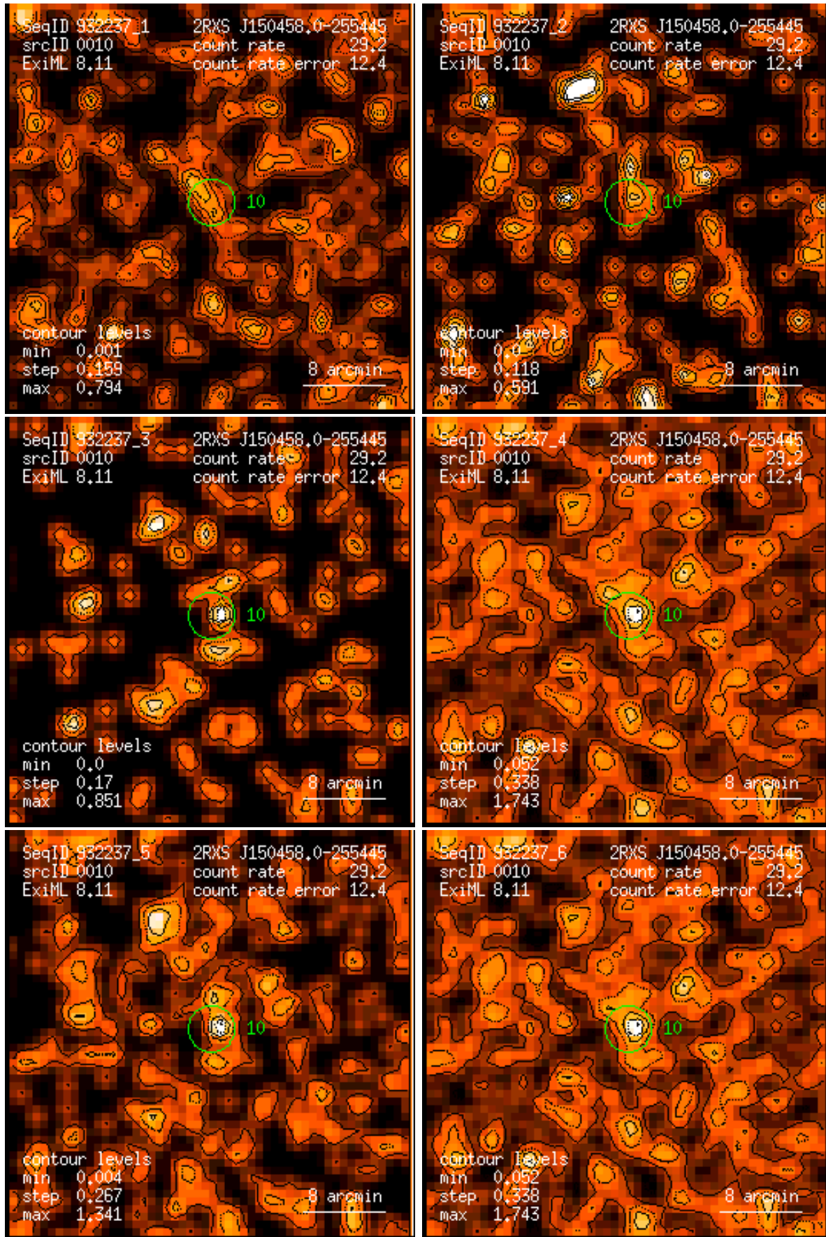
Figure 10: RASS 932237: detection 0010: band rate images, Gaussian filter: (1) PSPC channels 11 – 41, (2) 52 – 90, (3) 91 – 201, (4) 11 – 235, (5) 52 – 201, (6) 11 – 201. Broad band rates in counts/ks. Band rate contour levels in counts/ks/arcmin 2 .
