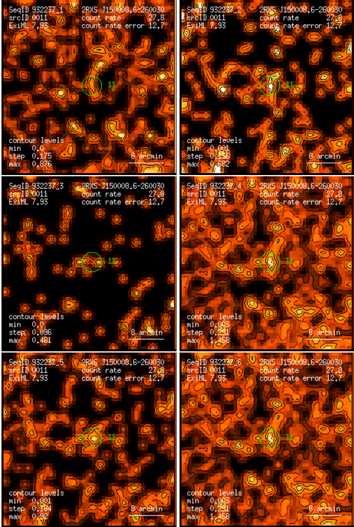
Figure 11: RASS 932237: detection 0011: band rate images, Gaussian filter: (1) PSPC channels 11 – 41, (2) 52 – 90, (3) 91 – 201, (4) 11 – 235, (5) 52 – 201, (6) 11 – 201. Broad band rates in counts/ks. Band rate contour levels in counts/ks/arcmin 2 .
