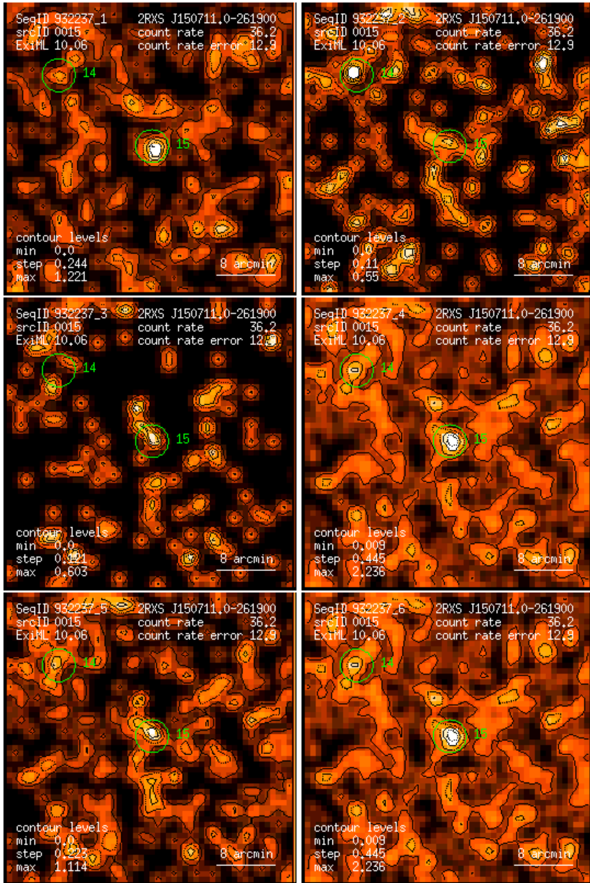
Figure 15: RASS 932237: detection 0015: band rate images, Gaussian filter: (1) PSPC channels 11 – 41, (2) 52 – 90, (3) 91 – 201, (4) 11 – 235, (5) 52 – 201, (6) 11 – 201. Broad band rates in counts/ks. Band rate contour levels in counts/ks/arcmin 2 .
