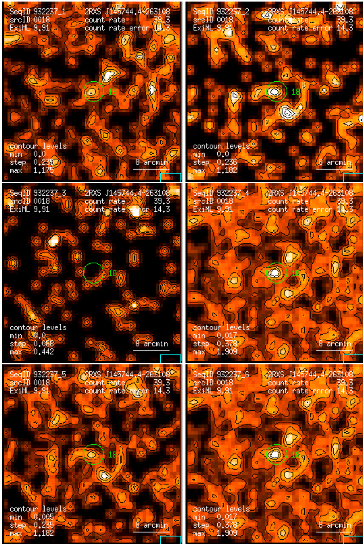
Figure 18: RASS 932237: detection 0018: band rate images, Gaussian filter: (1) PSPC channels 11 – 41, (2) 52 – 90, (3) 91 – 201, (4) 11 – 235, (5) 52 – 201, (6) 11 – 201. Broad band rates in counts/ks. Band rate contour levels in counts/ks/arcmin 2 .
