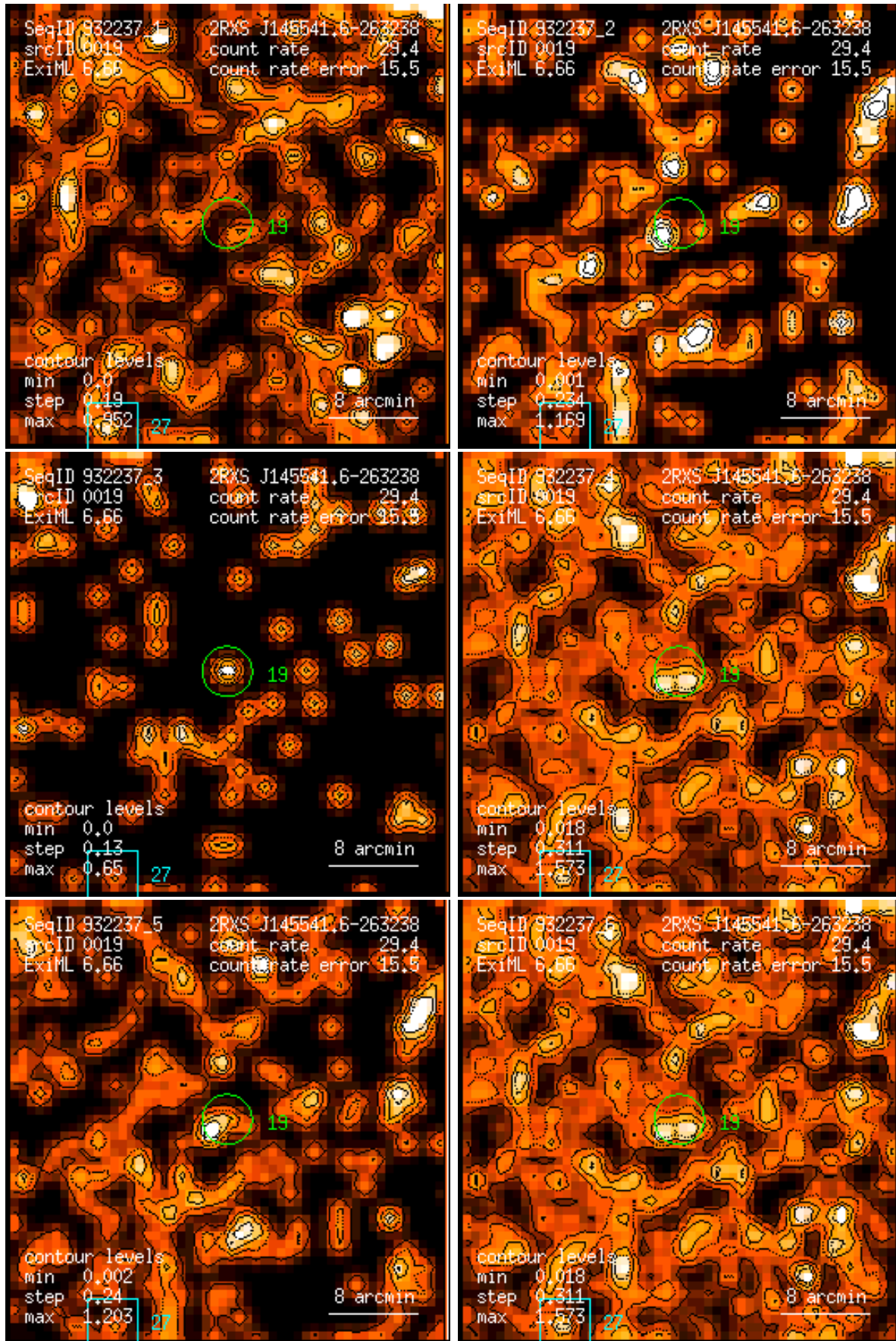
Figure 19: RASS 932237: detection 0019: band rate images, Gaussian filter: (1) PSPC channels 11 – 41, (2) 52 – 90, (3) 91 – 201, (4) 11 – 235, (5) 52 – 201, (6) 11 – 201. Broad band rates in counts/ks. Band rate contour levels in counts/ks/arcmin 2 .
