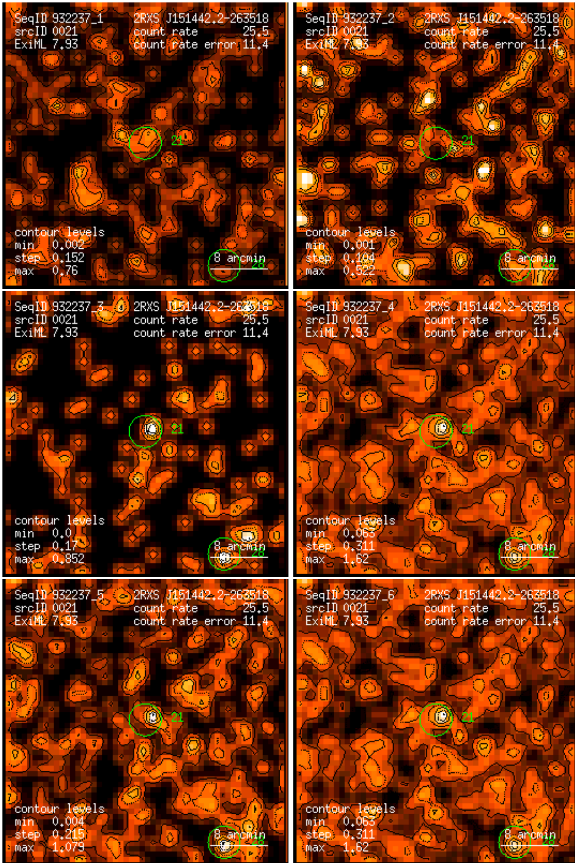
Figure 21: RASS 932237: detection 0021: band rate images, Gaussian filter: (1) PSPC channels 11 – 41, (2) 52 – 90, (3) 91 – 201, (4) 11 – 235, (5) 52 – 201, (6) 11 – 201. Broad band rates in counts/ks. Band rate contour levels in counts/ks/arcmin 2 .
