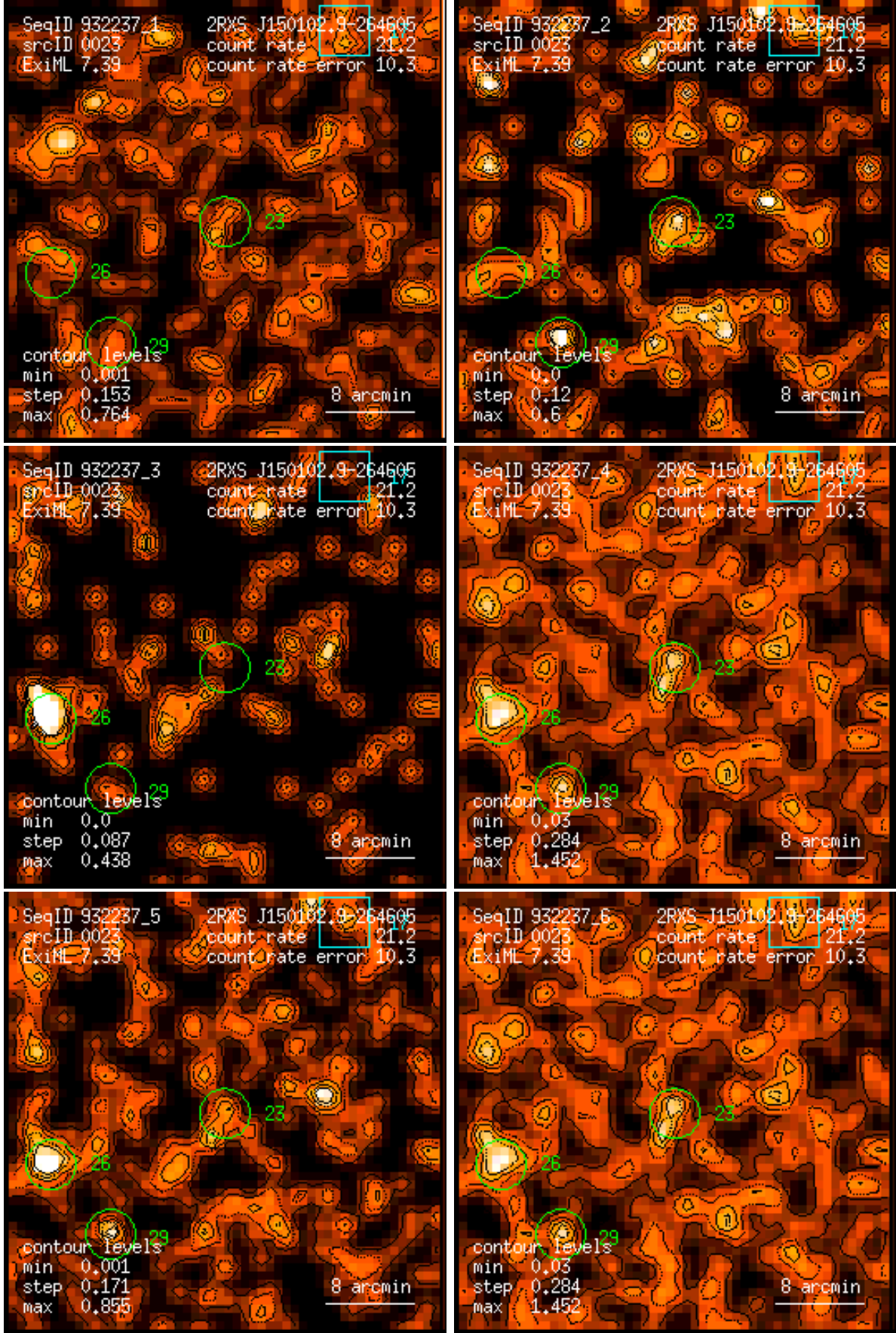
Figure 23: RASS 932237: detection 0023: band rate images, Gaussian filter: (1) PSPC channels 11 – 41, (2) 52 – 90, (3) 91 – 201, (4) 11 – 235, (5) 52 – 201, (6) 11 – 201. Broad band rates in counts/ks. Band rate contour levels in counts/ks/arcmin 2 .
