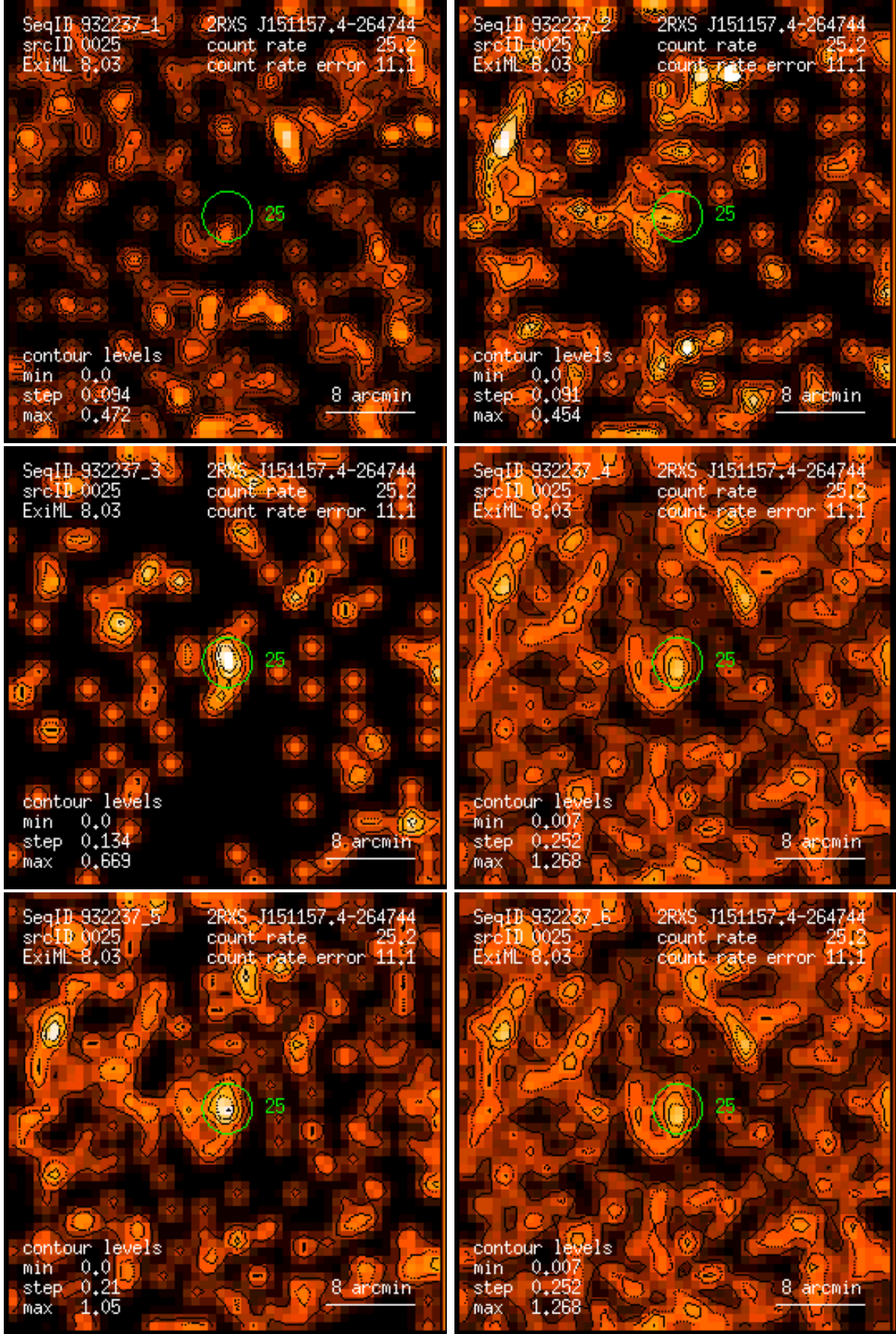
Figure 25: RASS 932237: detection 0025: band rate images, Gaussian filter: (1) PSPC channels 11 – 41, (2) 52 – 90, (3) 91 – 201, (4) 11 – 235, (5) 52 – 201, (6) 11 – 201. Broad band rates in counts/ks. Band rate contour levels in counts/ks/arcmin 2 .
