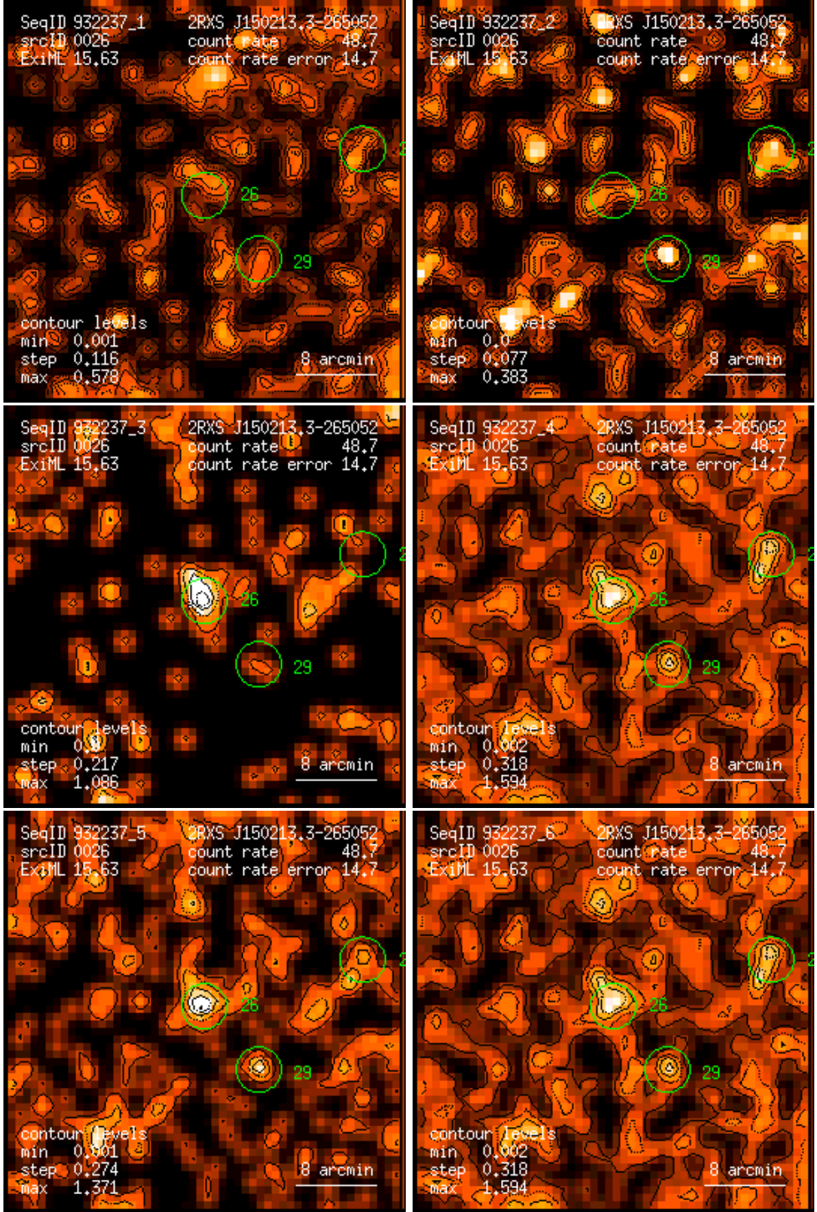
Figure 26: RASS 932237: detection 0026: band rate images, Gaussian filter: (1) PSPC channels 11 – 41, (2) 52 – 90, (3) 91 – 201, (4) 11 – 235, (5) 52 – 201, (6) 11 – 201. Broad band rates in counts/ks. Band rate contour levels in counts/ks/arcmin 2 .
