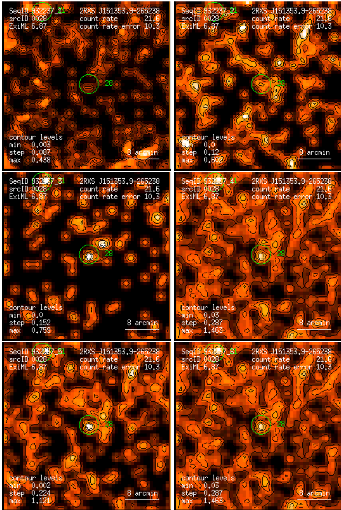
Figure 28: RASS 932237: detection 0028: band rate images, Gaussian filter: (1) PSPC channels 11 – 41, (2) 52 – 90, (3) 91 – 201, (4) 11 – 235, (5) 52 – 201, (6) 11 – 201. Broad band rates in counts/ks. Band rate contour levels in counts/ks/arcmin 2 .
