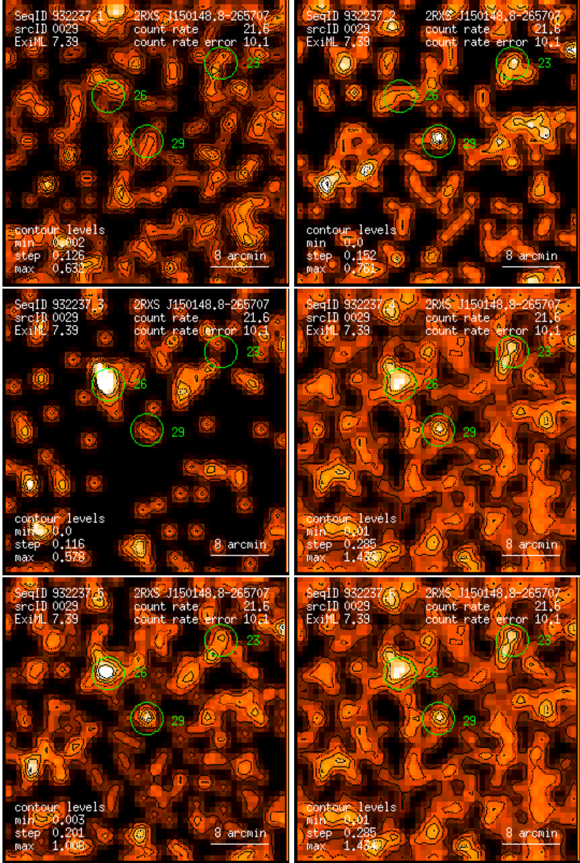
Figure 29: RASS 932237: detection 0029: band rate images, Gaussian filter: (1) PSPC channels 11 – 41, (2) 52 – 90, (3) 91 – 201, (4) 11 – 235, (5) 52 – 201, (6) 11 – 201. Broad band rates in counts/ks. Band rate contour levels in counts/ks/arcmin 2 .
