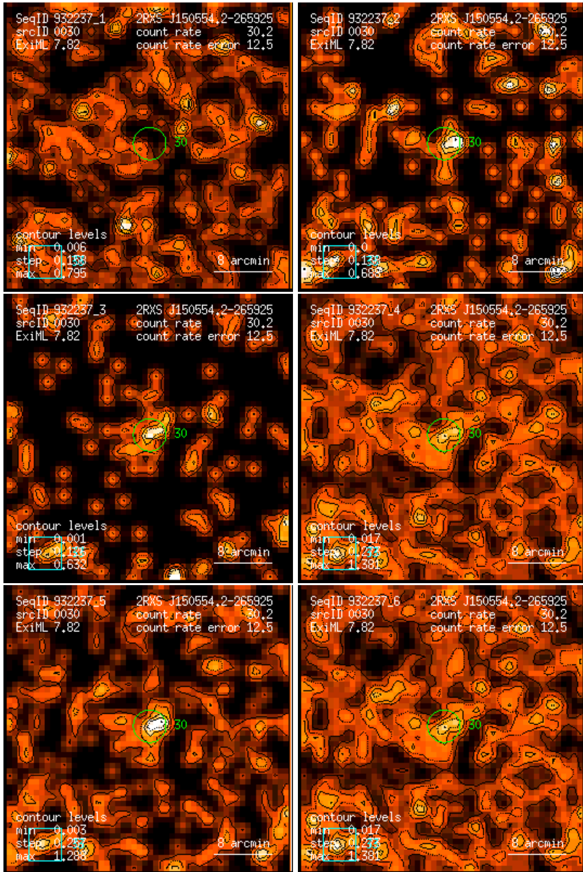
Figure 30: RASS 932237: detection 0030: band rate images, Gaussian filter: (1) PSPC channels 11 – 41, (2) 52 – 90, (3) 91 – 201, (4) 11 – 235, (5) 52 – 201, (6) 11 – 201. Broad band rates in counts/ks. Band rate contour levels in counts/ks/arcmin 2 .
